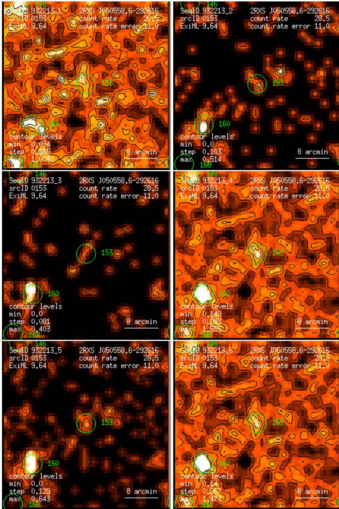
Figure 153: RASS 932213: detection 0153: band rate images, Gaussian filter: (1) PSPC channels 11 – 41, (2) 52 – 90, (3) 91 – 201, (4) 11 – 235, (5) 52 – 201, (6) 11 – 201. Broad band rates in counts/ks. Band rate contour levels in counts/ks/arcmin 2 .
