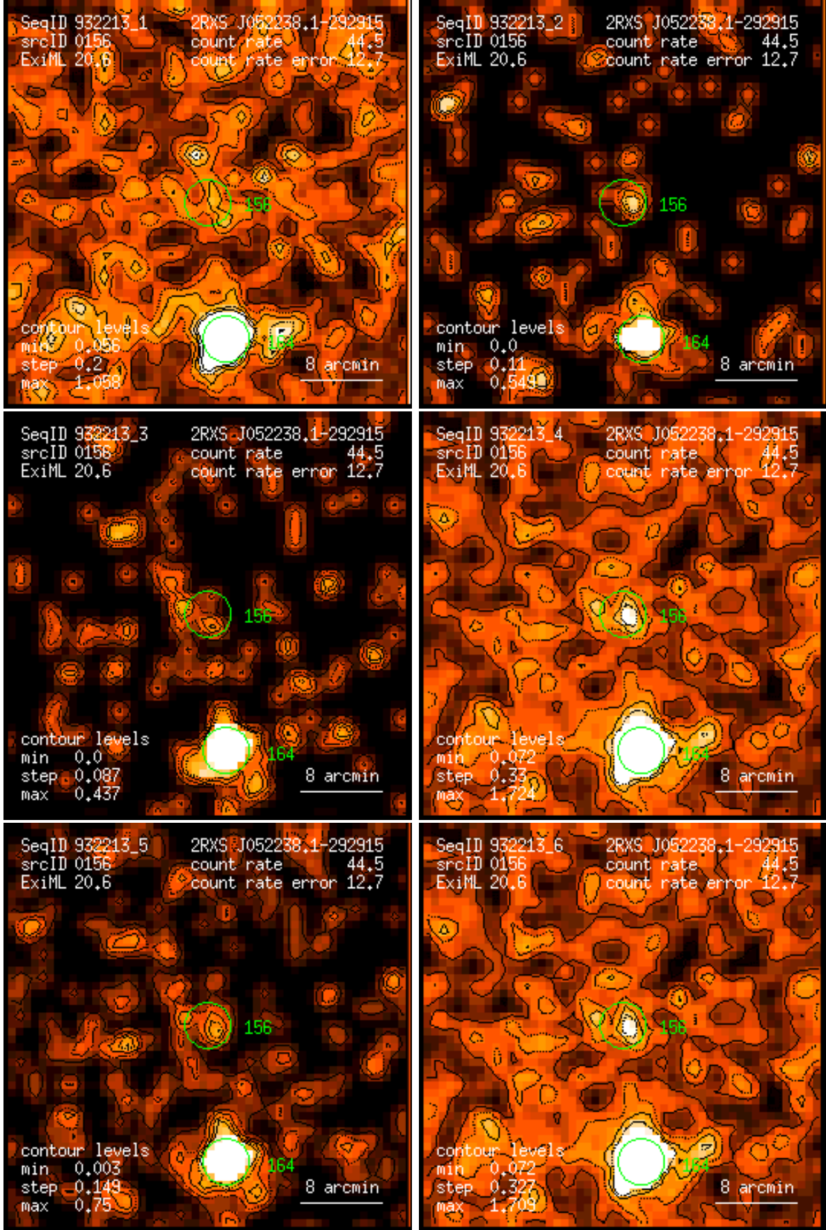
Figure 156: RASS 932213: detection 0156: band rate images, Gaussian filter: (1) PSPC channels 11 – 41, (2) 52 – 90, (3) 91 – 201, (4) 11 – 235, (5) 52 – 201, (6) 11 – 201. Broad band rates in counts/ks. Band rate contour levels in counts/ks/arcmin 2 .
