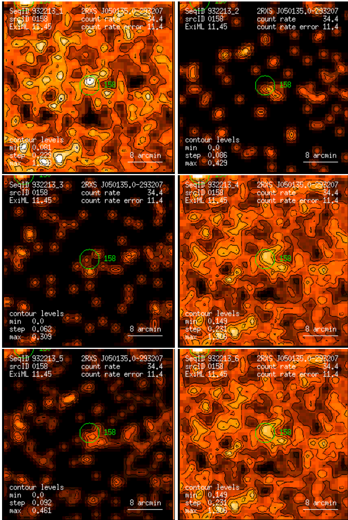
Figure 158: RASS 932213: detection 0158: band rate images, Gaussian filter: (1) PSPC channels 11 – 41, (2) 52 – 90, (3) 91 – 201, (4) 11 – 235, (5) 52 – 201, (6) 11 – 201. Broad band rates in counts/ks. Band rate contour levels in counts/ks/arcmin 2 .
