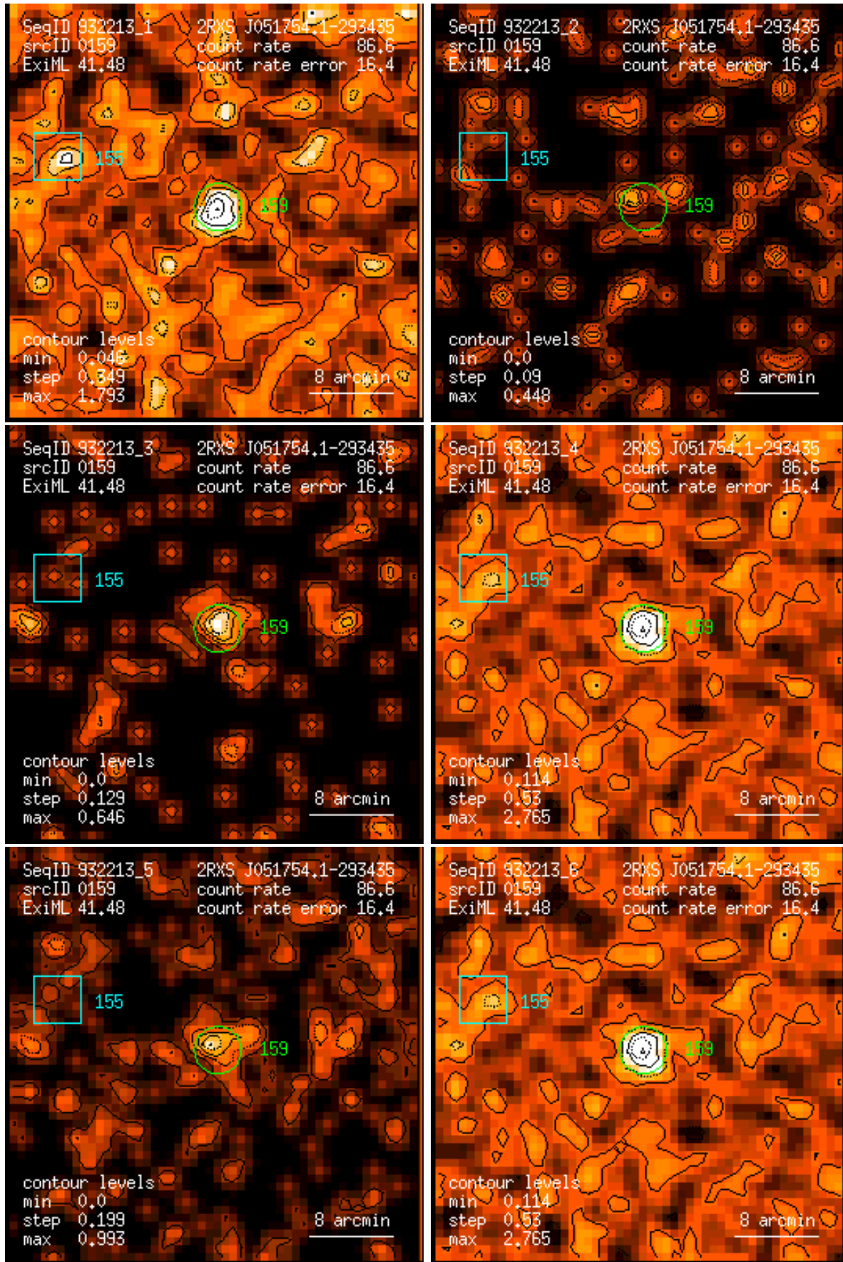
Figure 159: RASS 932213: detection 0159: band rate images, Gaussian filter: (1) PSPC channels 11 – 41, (2) 52 – 90, (3) 91 – 201, (4) 11 – 235, (5) 52 – 201, (6) 11 – 201. Broad band rates in counts/ks. Band rate contour levels in counts/ks/arcmin 2 .
