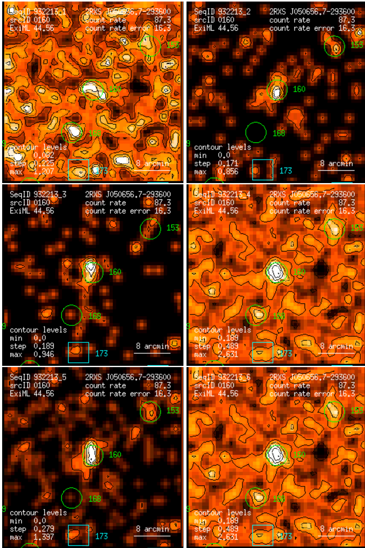
Figure 160: RASS 932213: detection 0160: band rate images, Gaussian filter: (1) PSPC channels 11 – 41, (2) 52 – 90, (3) 91 – 201, (4) 11 – 235, (5) 52 – 201, (6) 11 – 201. Broad band rates in counts/ks. Band rate contour levels in counts/ks/arcmin 2 .
