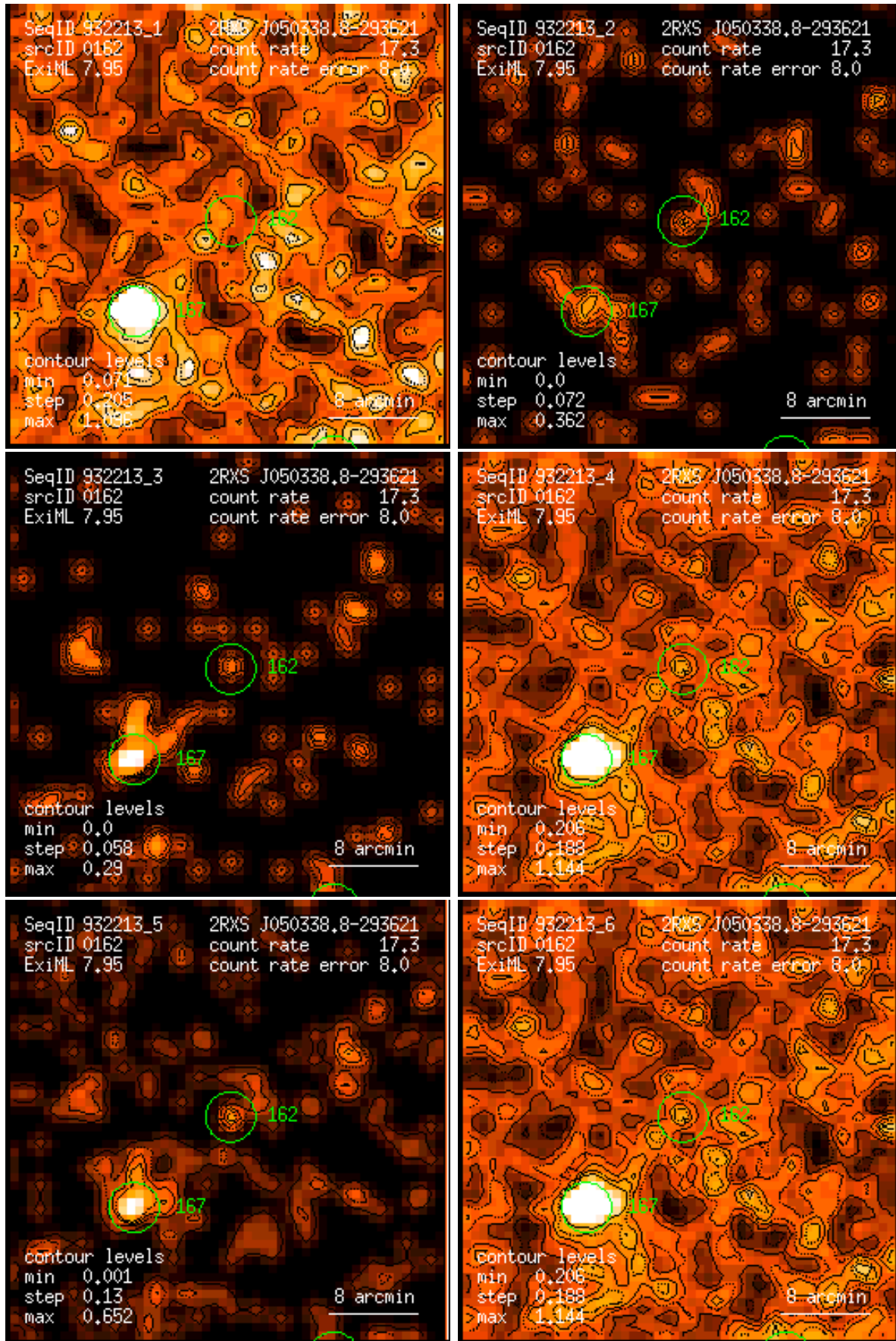
Figure 162: RASS 932213: detection 0162: band rate images, Gaussian filter: (1) PSPC channels 11 – 41, (2) 52 – 90, (3) 91 – 201, (4) 11 – 235, (5) 52 – 201, (6) 11 – 201. Broad band rates in counts/ks. Band rate contour levels in counts/ks/arcmin 2 .
