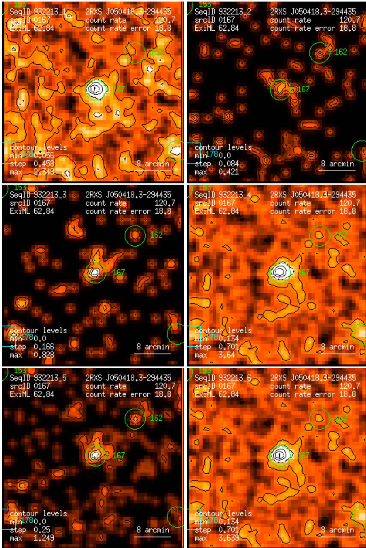
Figure 167: RASS 932213: detection 0167: band rate images, Gaussian filter: (1) PSPC channels 11 – 41, (2) 52 – 90, (3) 91 – 201, (4) 11 – 235, (5) 52 – 201, (6) 11 – 201. Broad band rates in counts/ks. Band rate contour levels in counts/ks/arcmin 2 .
