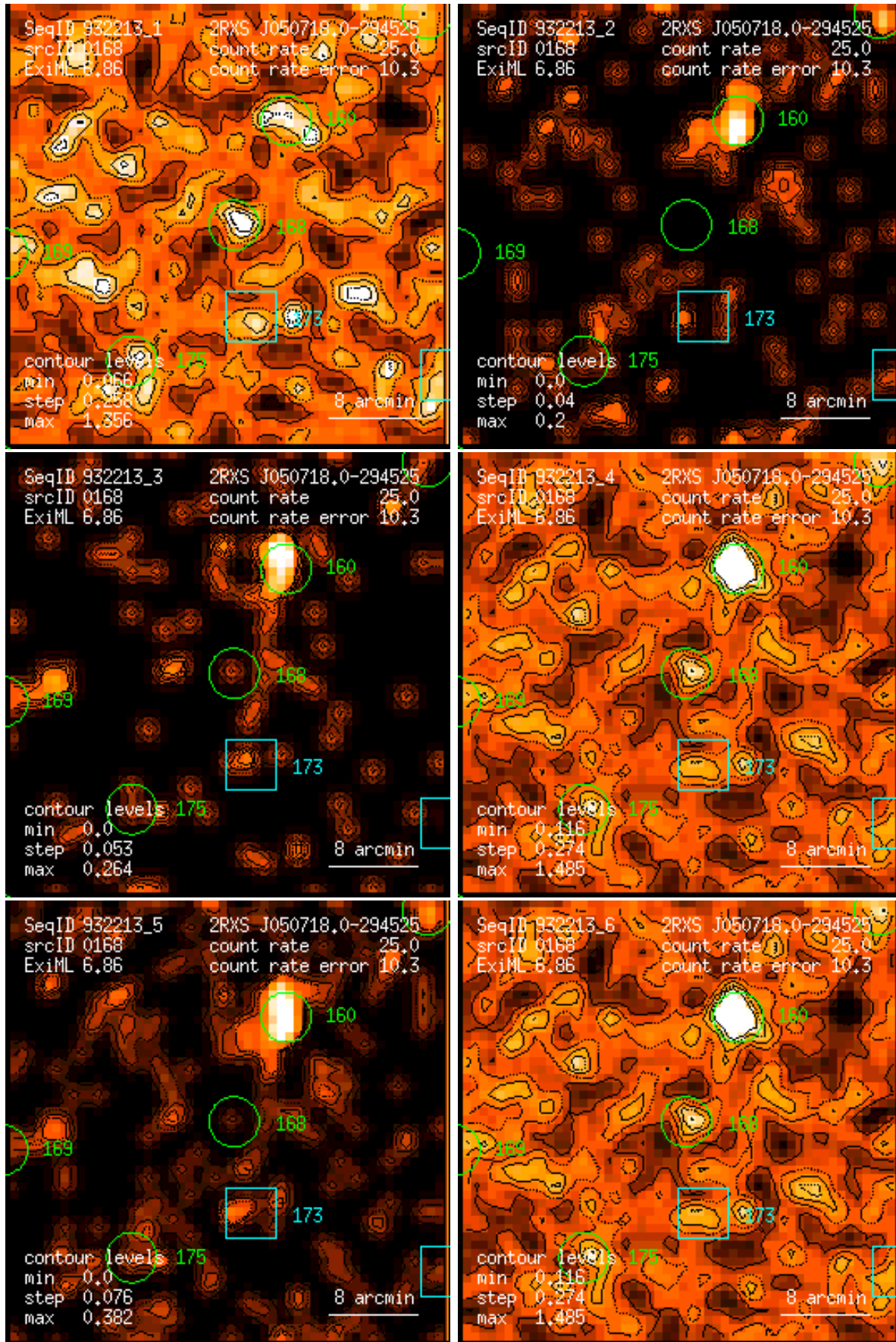
Figure 168: RASS 932213: detection 0168: band rate images, Gaussian filter: (1) PSPC channels 11 – 41, (2) 52 – 90, (3) 91 – 201, (4) 11 – 235, (5) 52 – 201, (6) 11 – 201. Broad band rates in counts/ks. Band rate contour levels in counts/ks/arcmin 2 .
