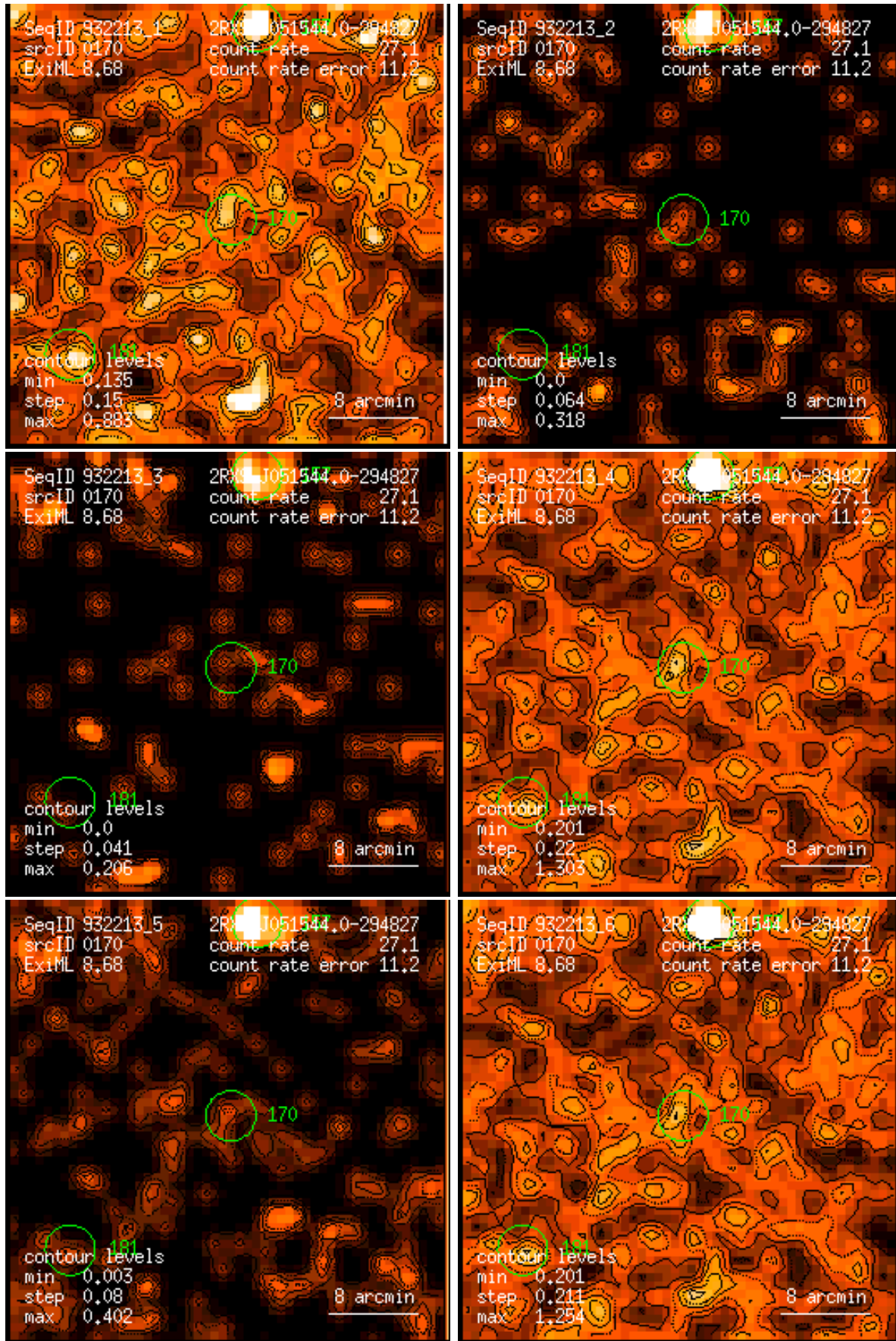
Figure 170: RASS 932213: detection 0170: band rate images, Gaussian filter: (1) PSPC channels 11 – 41, (2) 52 – 90, (3) 91 – 201, (4) 11 – 235, (5) 52 – 201, (6) 11 – 201. Broad band rates in counts/ks. Band rate contour levels in counts/ks/arcmin 2 .
