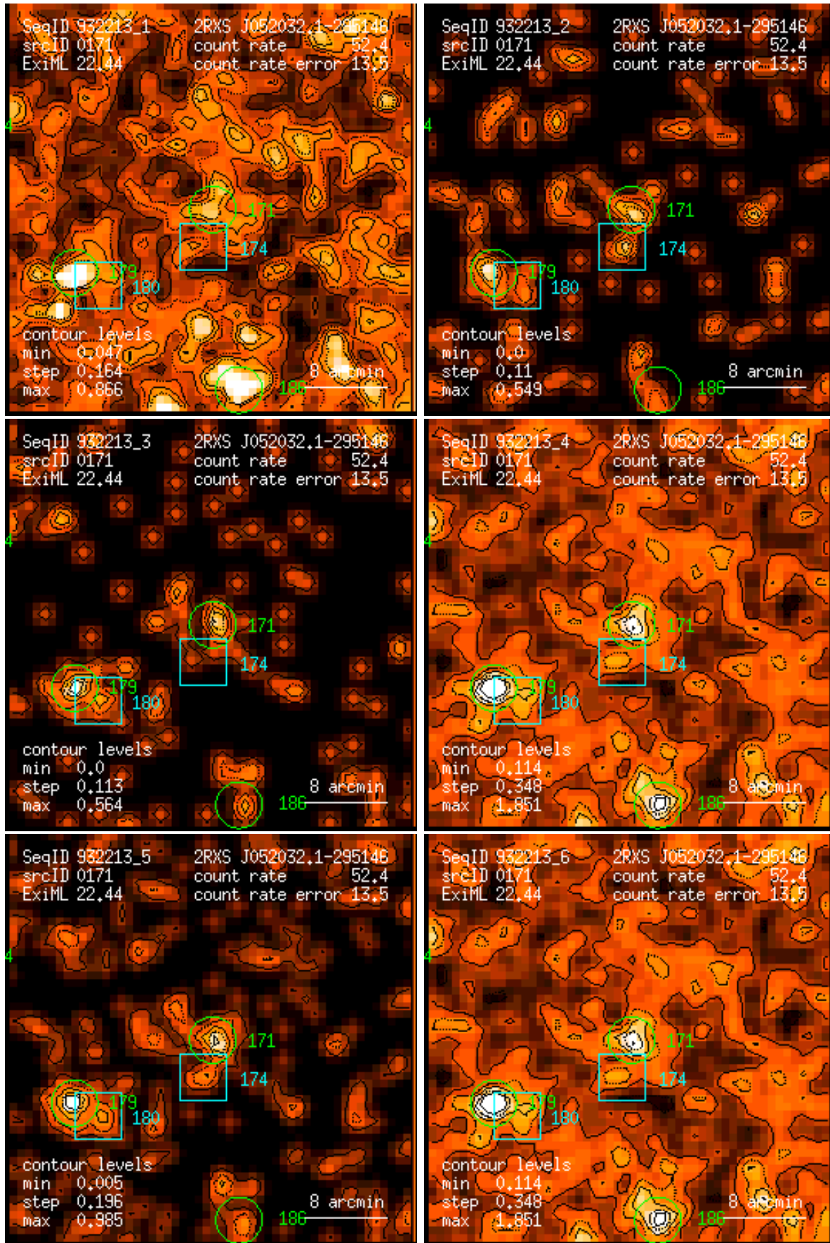
Figure 171: RASS 932213: detection 0171: band rate images, Gaussian filter: (1) PSPC channels 11 – 41, (2) 52 – 90, (3) 91 – 201, (4) 11 – 235, (5) 52 – 201, (6) 11 – 201. Broad band rates in counts/ks. Band rate contour levels in counts/ks/arcmin 2 .
