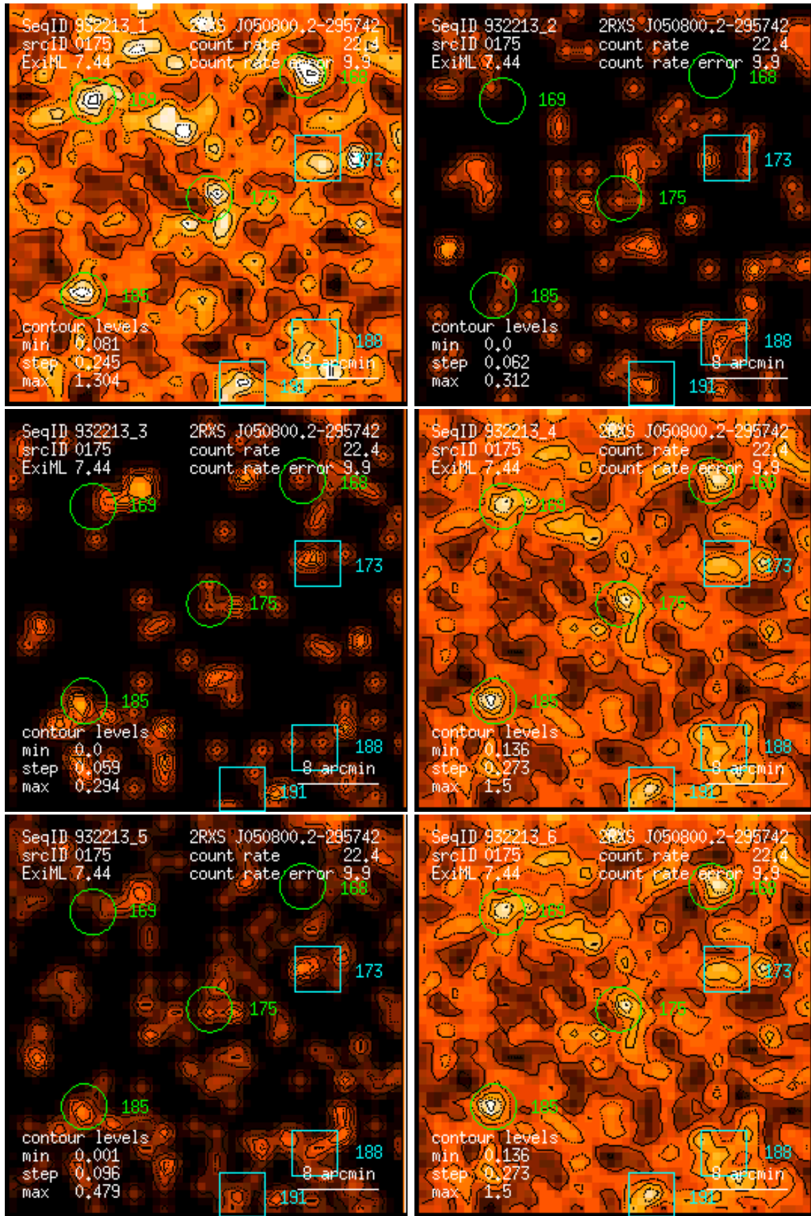
Figure 175: RASS 932213: detection 0175: band rate images, Gaussian filter: (1) PSPC channels 11 – 41, (2) 52 – 90, (3) 91 – 201, (4) 11 – 235, (5) 52 – 201, (6) 11 – 201. Broad band rates in counts/ks. Band rate contour levels in counts/ks/arcmin 2 .
