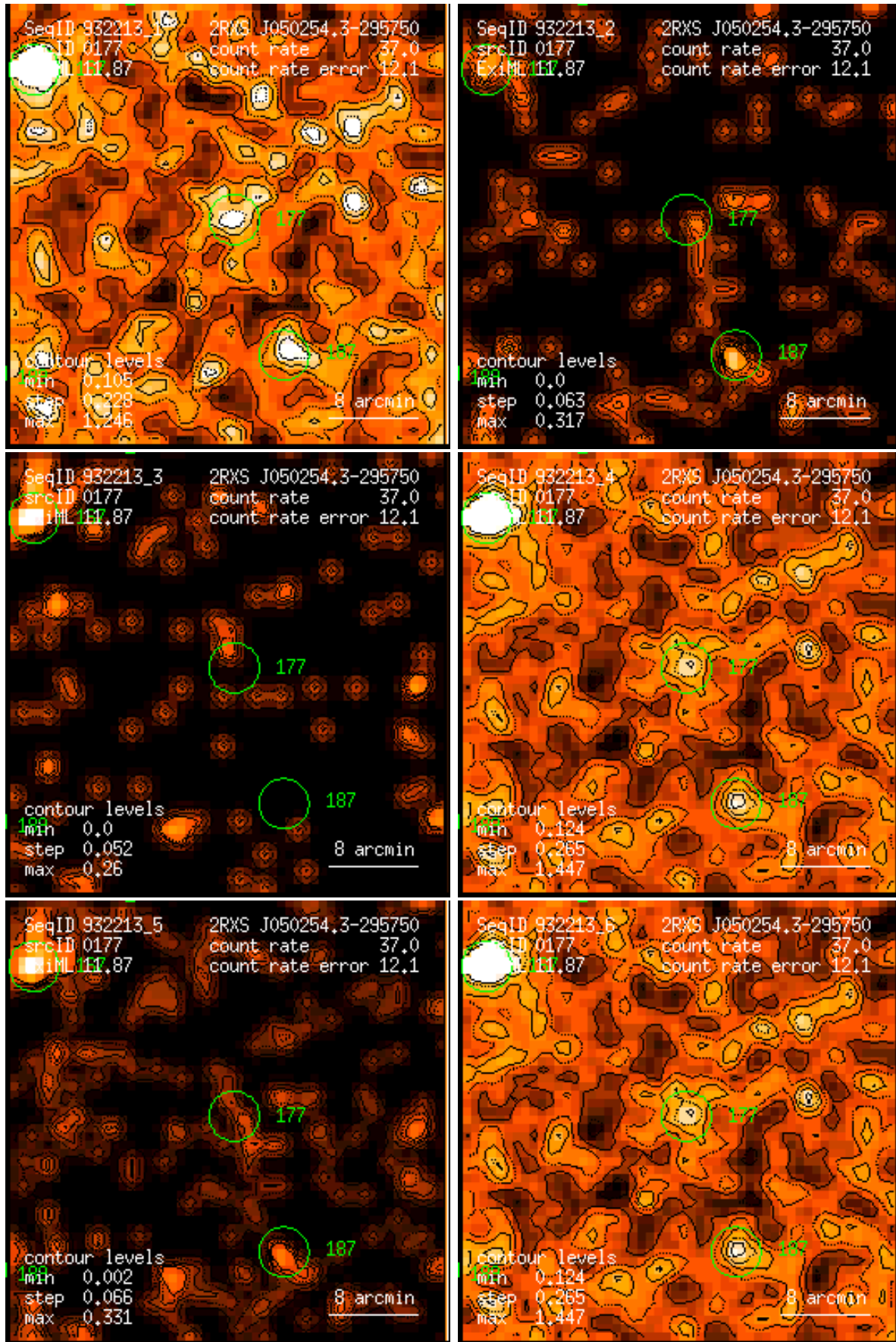
Figure 177: RASS 932213: detection 0177: band rate images, Gaussian filter: (1) PSPC channels 11 – 41, (2) 52 – 90, (3) 91 – 201, (4) 11 – 235, (5) 52 – 201, (6) 11 – 201. Broad band rates in counts/ks. Band rate contour levels in counts/ks/arcmin 2 .
