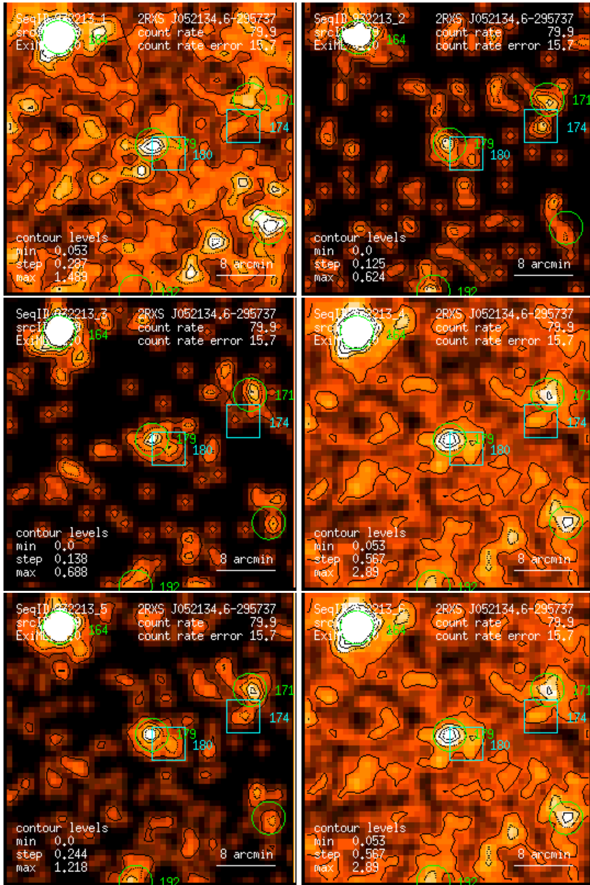
Figure 179: RASS 932213: detection 0179: band rate images, Gaussian filter: (1) PSPC channels 11 – 41, (2) 52 – 90, (3) 91 – 201, (4) 11 – 235, (5) 52 – 201, (6) 11 – 201. Broad band rates in counts/ks. Band rate contour levels in counts/ks/arcmin 2 .
