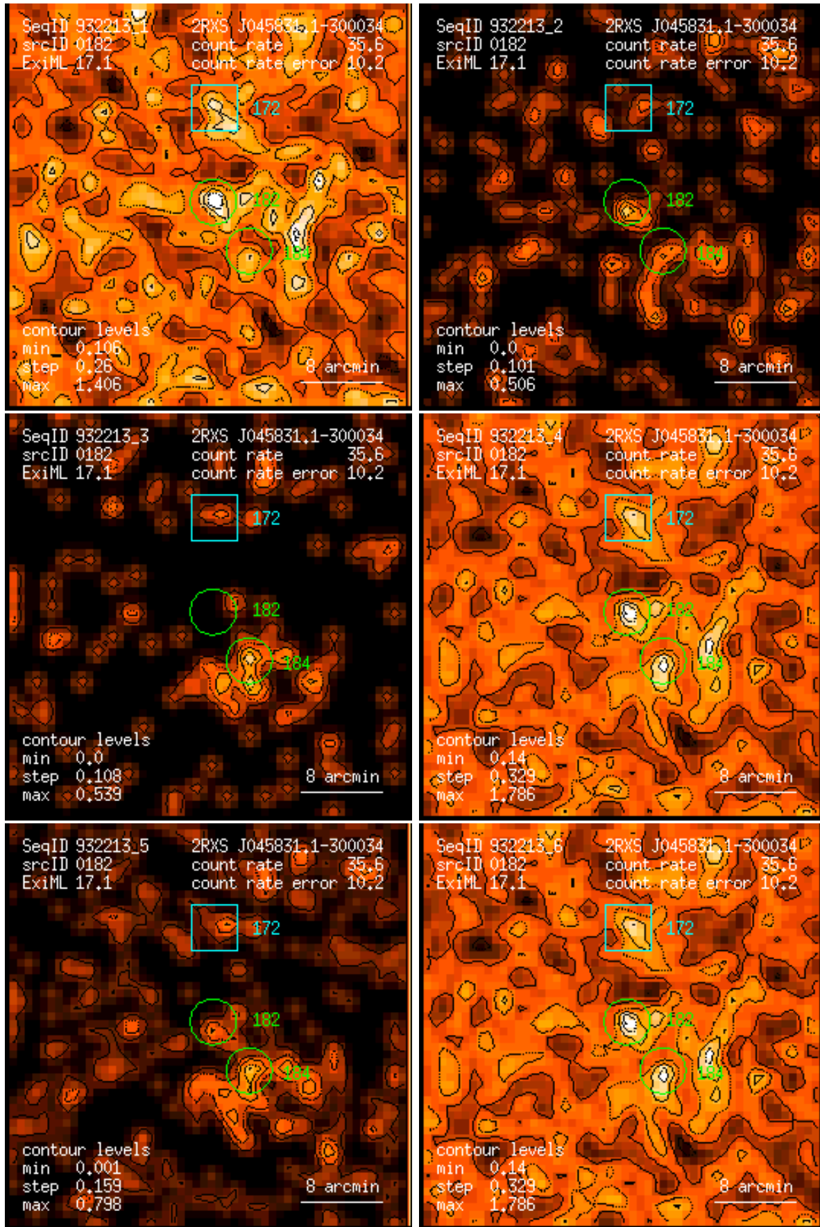
Figure 182: RASS 932213: detection 0182: band rate images, Gaussian filter: (1) PSPC channels 11 – 41, (2) 52 – 90, (3) 91 – 201, (4) 11 – 235, (5) 52 – 201, (6) 11 – 201. Broad band rates in counts/ks. Band rate contour levels in counts/ks/arcmin 2 .
