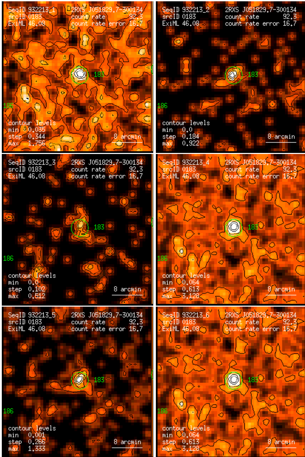
Figure 183: RASS 932213: detection 0183: band rate images, Gaussian filter: (1) PSPC channels 11 – 41, (2) 52 – 90, (3) 91 – 201, (4) 11 – 235, (5) 52 – 201, (6) 11 – 201. Broad band rates in counts/ks. Band rate contour levels in counts/ks/arcmin 2 .
