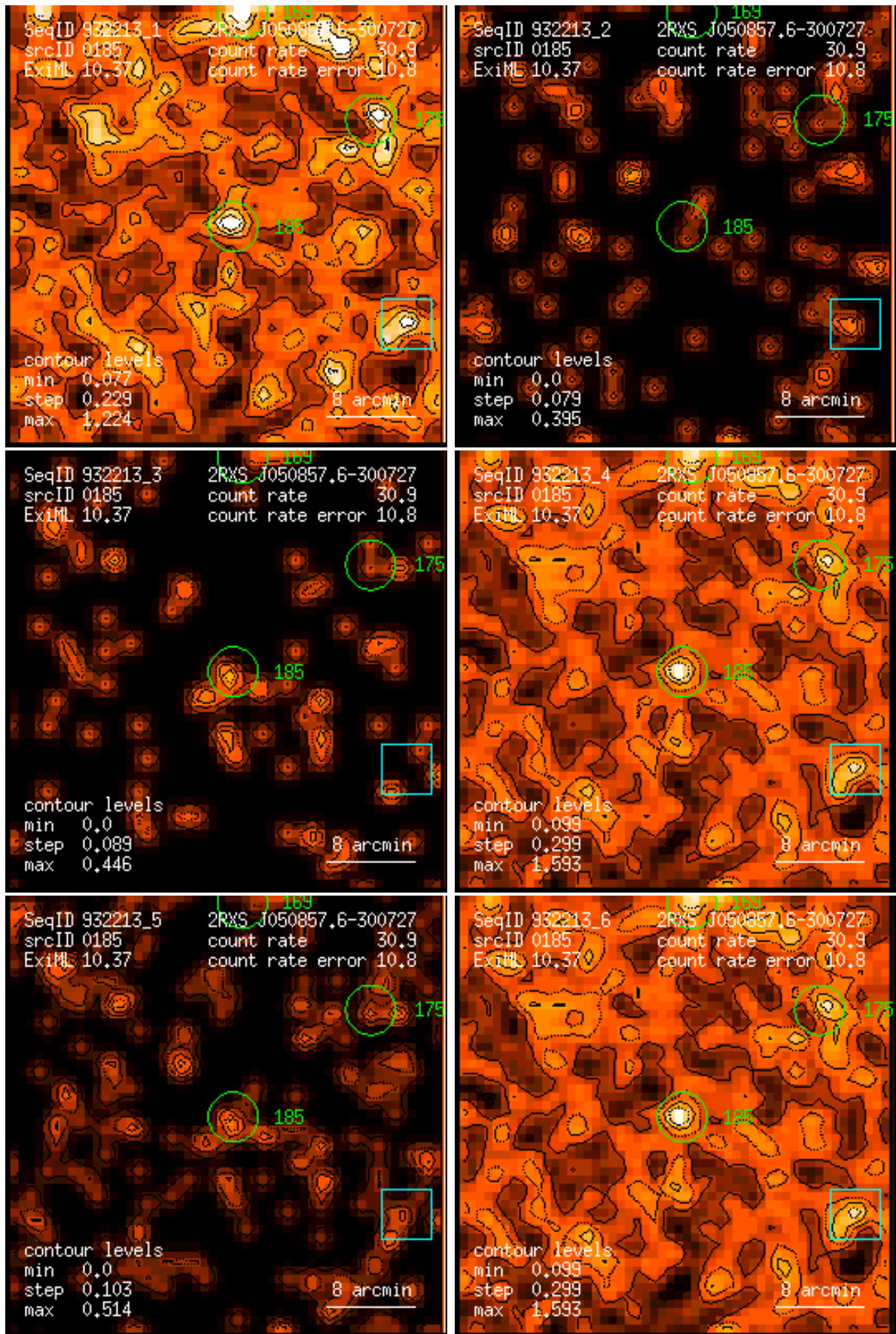
Figure 185: RASS 932213: detection 0185: band rate images, Gaussian filter: (1) PSPC channels 11 – 41, (2) 52 – 90, (3) 91 – 201, (4) 11 – 235, (5) 52 – 201, (6) 11 – 201. Broad band rates in counts/ks. Band rate contour levels in counts/ks/arcmin 2 .
