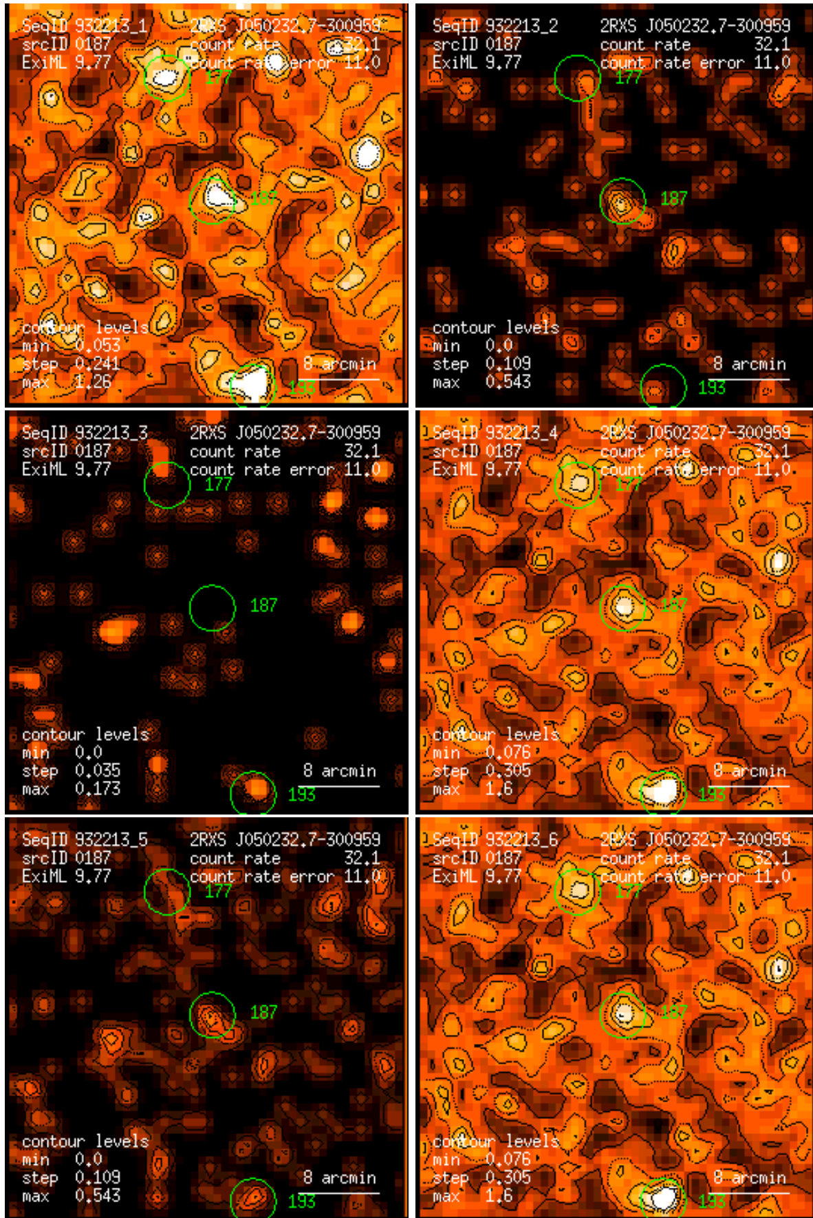
Figure 187: RASS 932213: detection 0187: band rate images, Gaussian filter: (1) PSPC channels 11 – 41, (2) 52 – 90, (3) 91 – 201, (4) 11 – 235, (5) 52 – 201, (6) 11 – 201. Broad band rates in counts/ks. Band rate contour levels in counts/ks/arcmin 2 .
