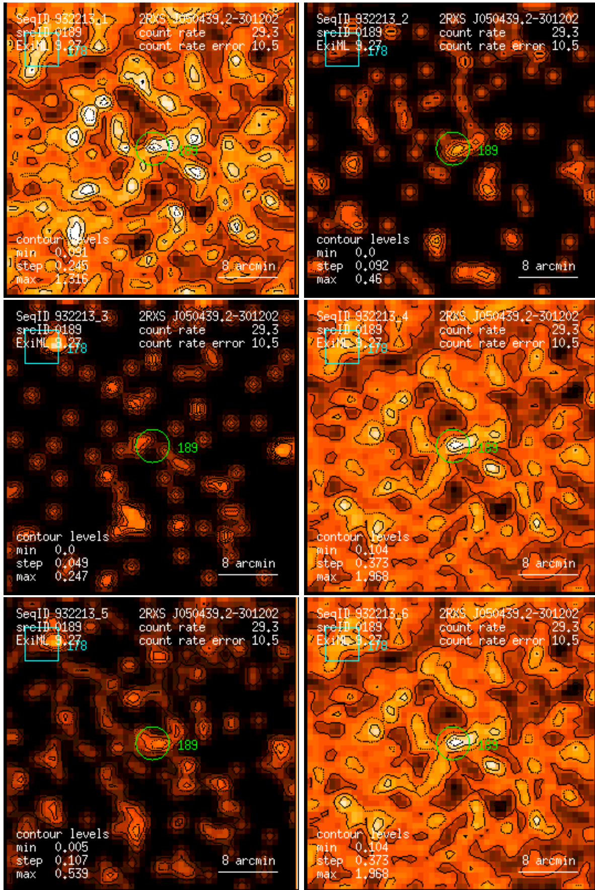
Figure 189: RASS 932213: detection 0189: band rate images, Gaussian filter: (1) PSPC channels 11 – 41, (2) 52 – 90, (3) 91 – 201, (4) 11 – 235, (5) 52 – 201, (6) 11 – 201. Broad band rates in counts/ks. Band rate contour levels in counts/ks/arcmin 2 .
