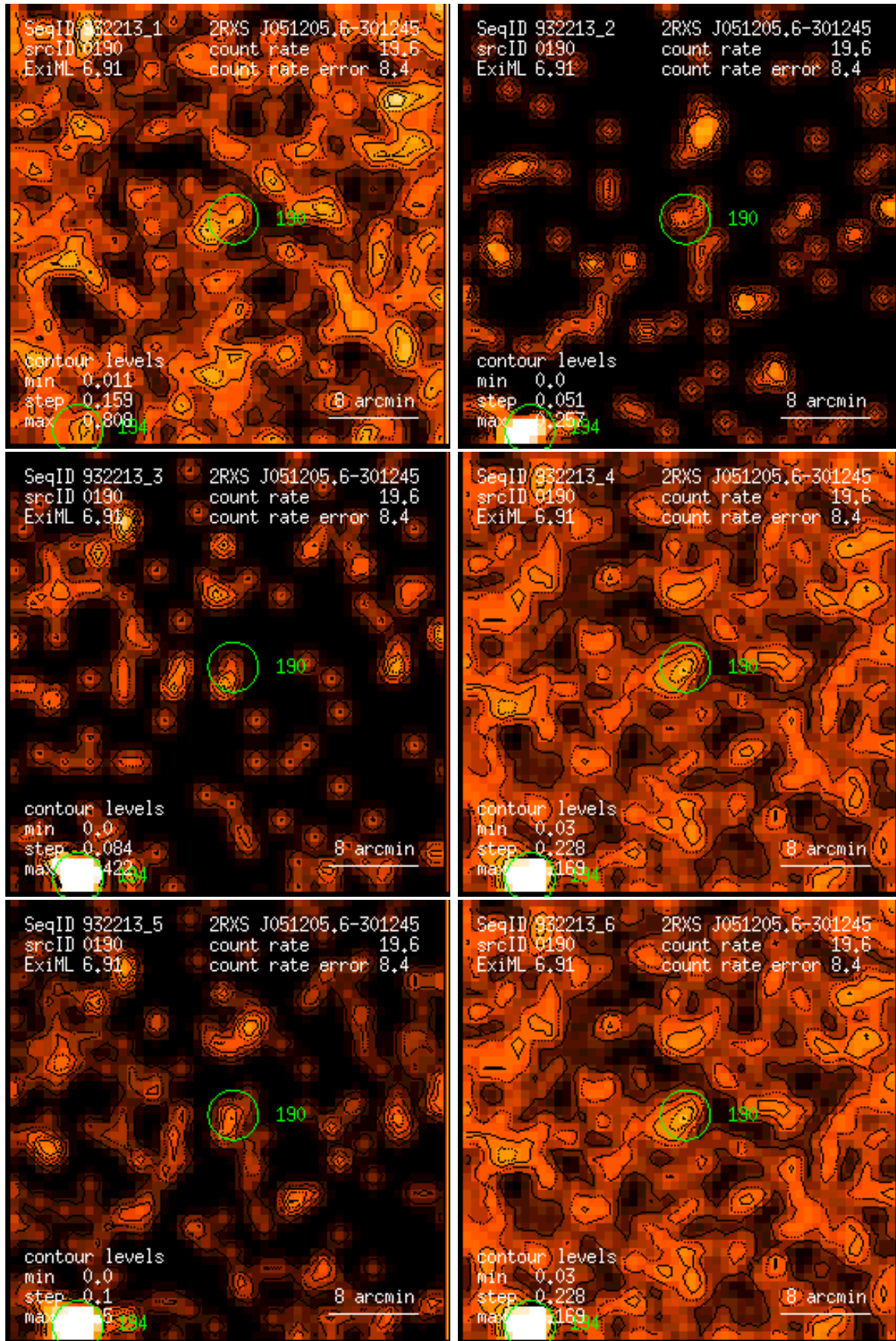
Figure 190: RASS 932213: detection 0190: band rate images, Gaussian filter: (1) PSPC channels 11 – 41, (2) 52 – 90, (3) 91 – 201, (4) 11 – 235, (5) 52 – 201, (6) 11 – 201. Broad band rates in counts/ks. Band rate contour levels in counts/ks/arcmin 2 .
