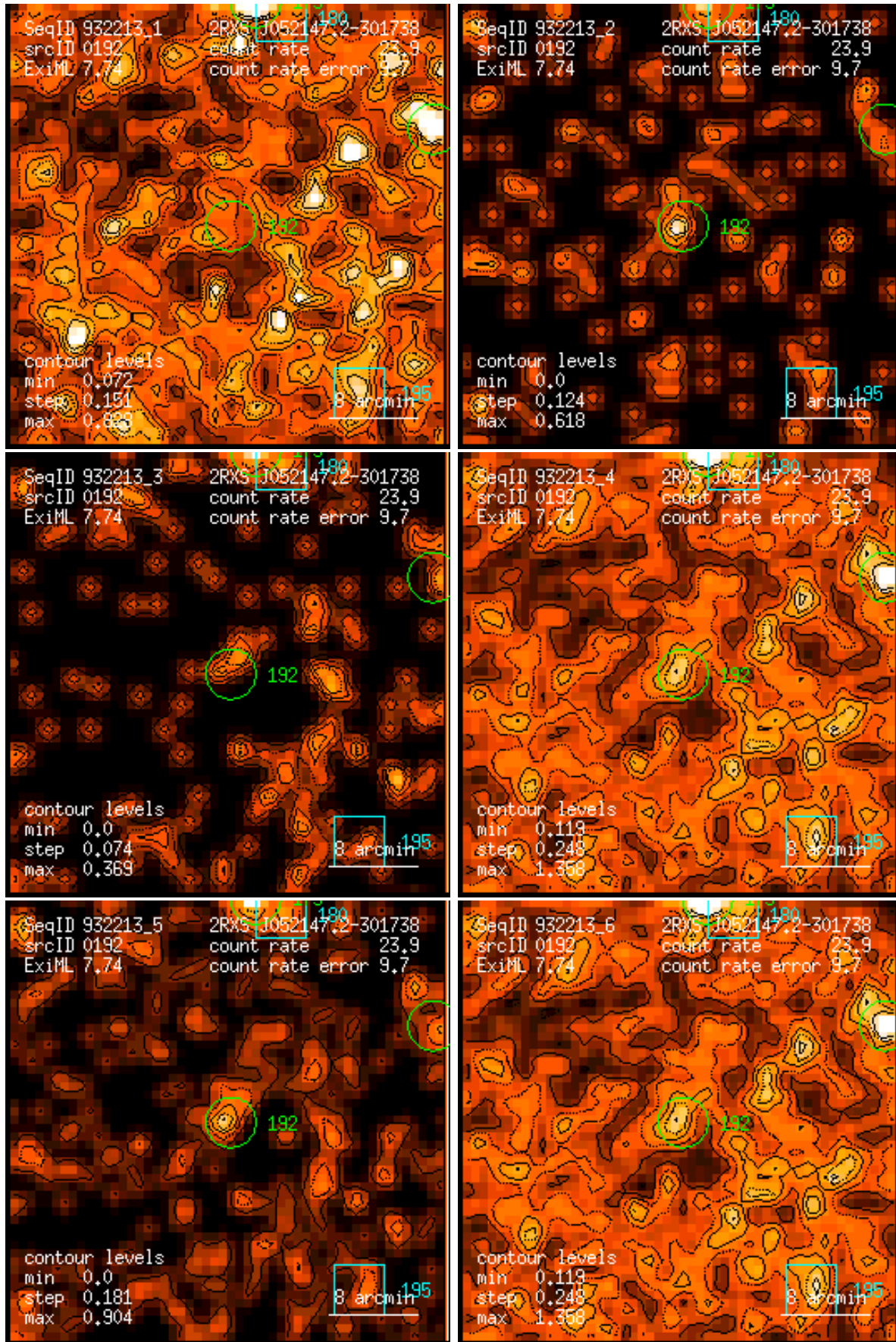
Figure 192: RASS 932213: detection 0192: band rate images, Gaussian filter: (1) PSPC channels 11 – 41, (2) 52 – 90, (3) 91 – 201, (4) 11 – 235, (5) 52 – 201, (6) 11 – 201. Broad band rates in counts/ks. Band rate contour levels in counts/ks/arcmin 2 .
