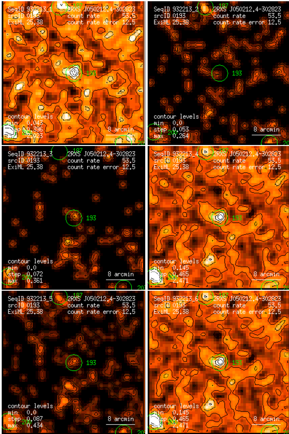
Figure 193: RASS 932213: detection 0193: band rate images, Gaussian filter: (1) PSPC channels 11 – 41, (2) 52 – 90, (3) 91 – 201, (4) 11 – 235, (5) 52 – 201, (6) 11 – 201. Broad band rates in counts/ks. Band rate contour levels in counts/ks/arcmin 2 .
