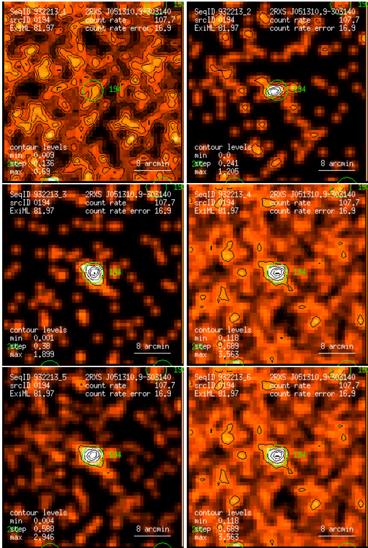
Figure 194: RASS 932213: detection 0194: band rate images, Gaussian filter: (1) PSPC channels 11 – 41, (2) 52 – 90, (3) 91 – 201, (4) 11 – 235, (5) 52 – 201, (6) 11 – 201. Broad band rates in counts/ks. Band rate contour levels in counts/ks/arcmin 2 .
