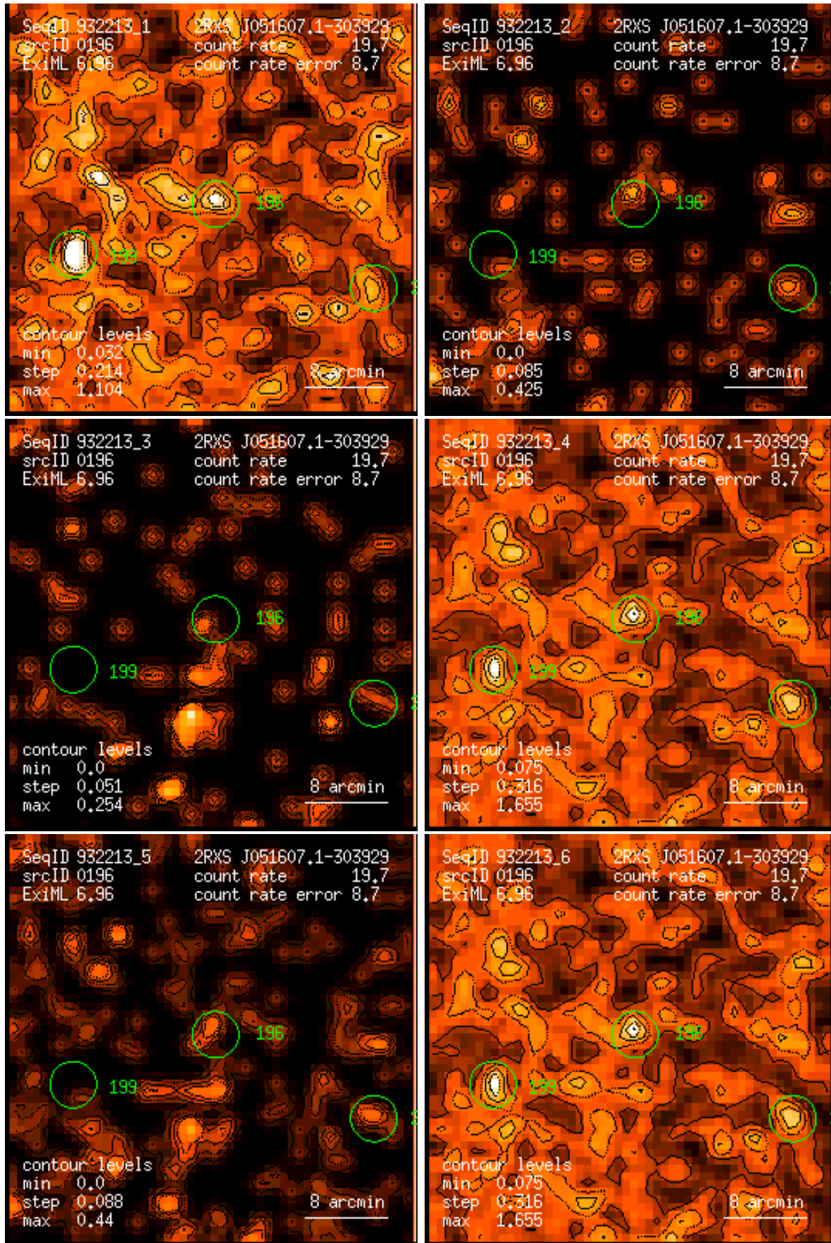
Figure 196: RASS 932213: detection 0196: band rate images, Gaussian filter: (1) PSPC channels 11 – 41, (2) 52 – 90, (3) 91 – 201, (4) 11 – 235, (5) 52 – 201, (6) 11 – 201. Broad band rates in counts/ks. Band rate contour levels in counts/ks/arcmin 2 .
