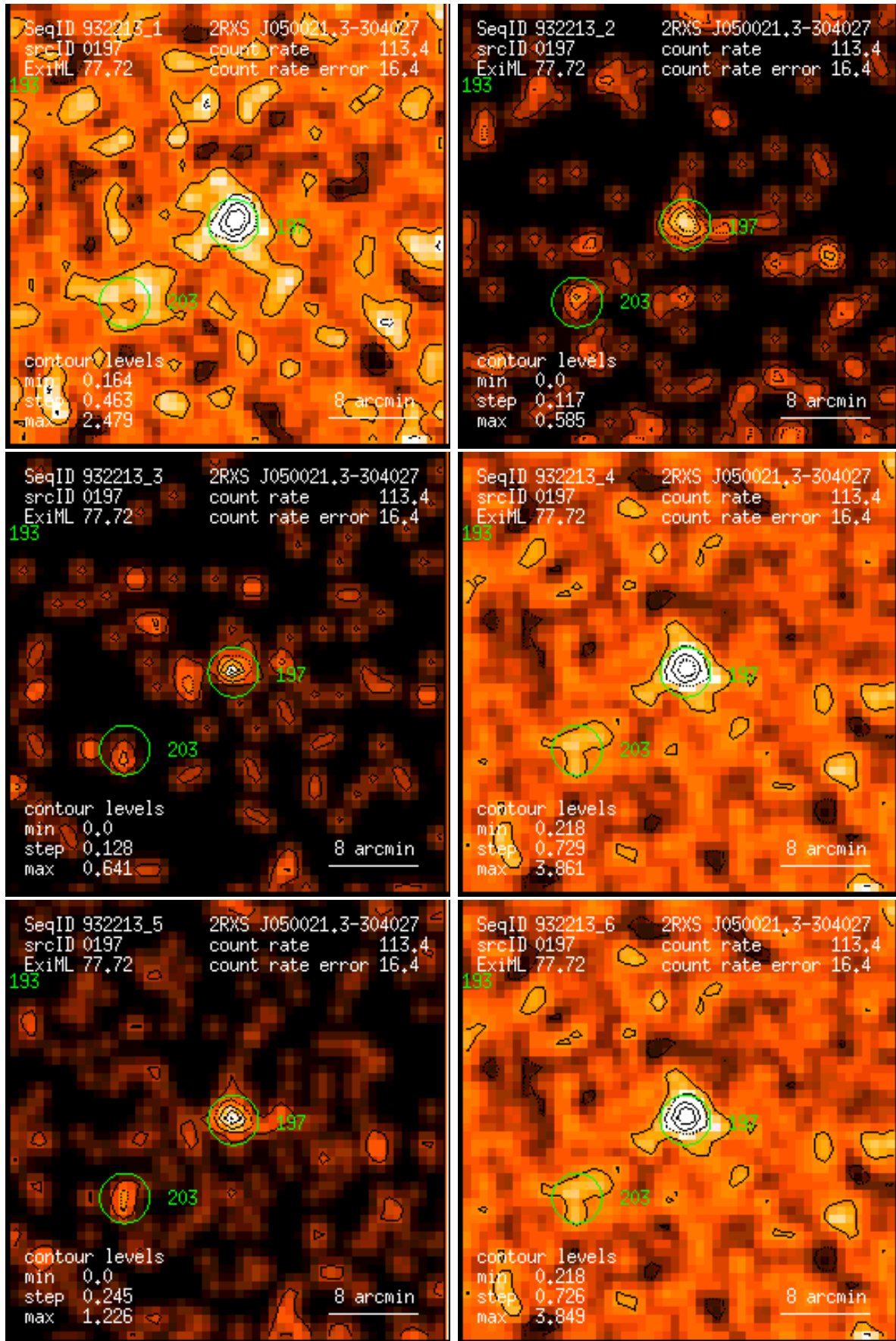
Figure 197: RASS 932213: detection 0197: band rate images, Gaussian filter: (1) PSPC channels 11 – 41, (2) 52 – 90, (3) 91 – 201, (4) 11 – 235, (5) 52 – 201, (6) 11 – 201. Broad band rates in counts/ks. Band rate contour levels in counts/ks/arcmin 2 .
