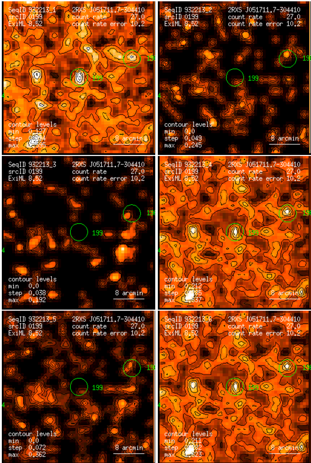
Figure 199: RASS 932213: detection 0199: band rate images, Gaussian filter: (1) PSPC channels 11 – 41, (2) 52 – 90, (3) 91 – 201, (4) 11 – 235, (5) 52 – 201, (6) 11 – 201. Broad band rates in counts/ks. Band rate contour levels in counts/ks/arcmin 2 .
