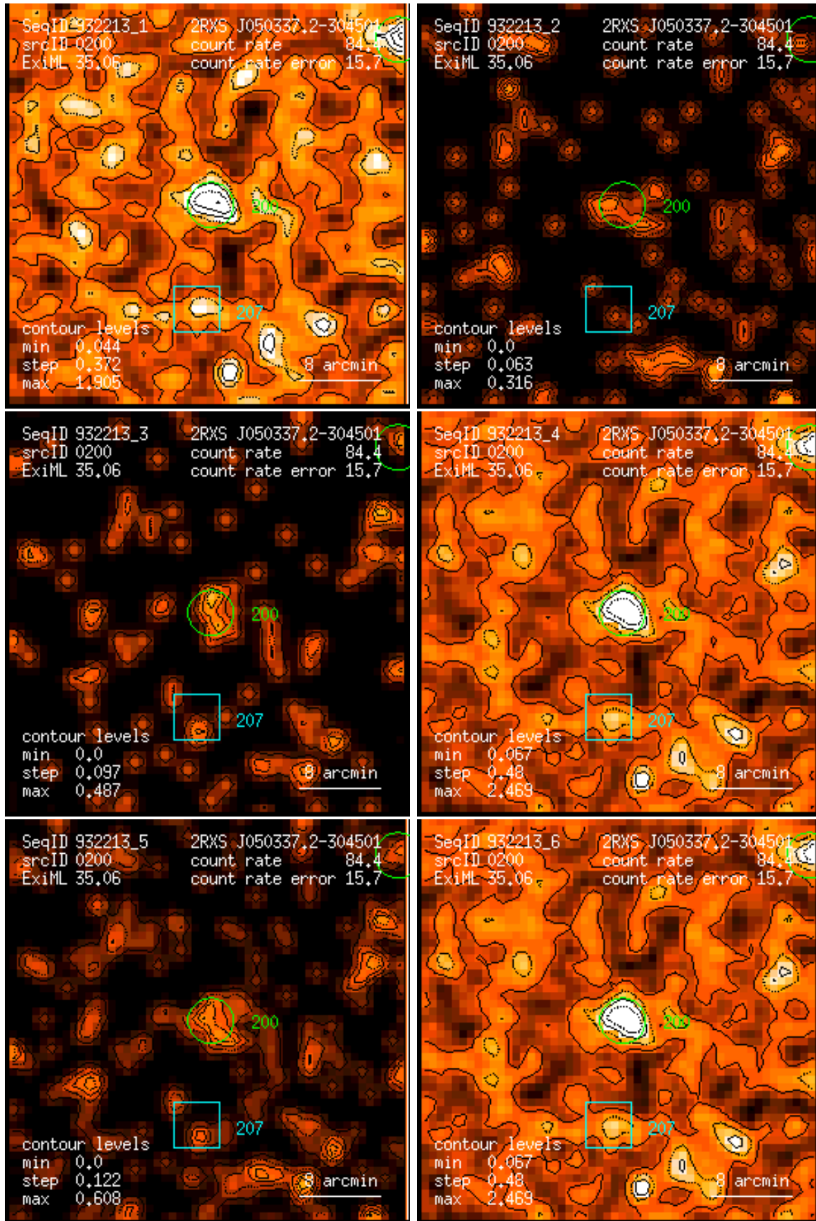
Figure 200: RASS 932213: detection 0200: band rate images, Gaussian filter: (1) PSPC channels 11 – 41, (2) 52 – 90, (3) 91 – 201, (4) 11 – 235, (5) 52 – 201, (6) 11 – 201. Broad band rates in counts/ks. Band rate contour levels in counts/ks/arcmin 2 .
