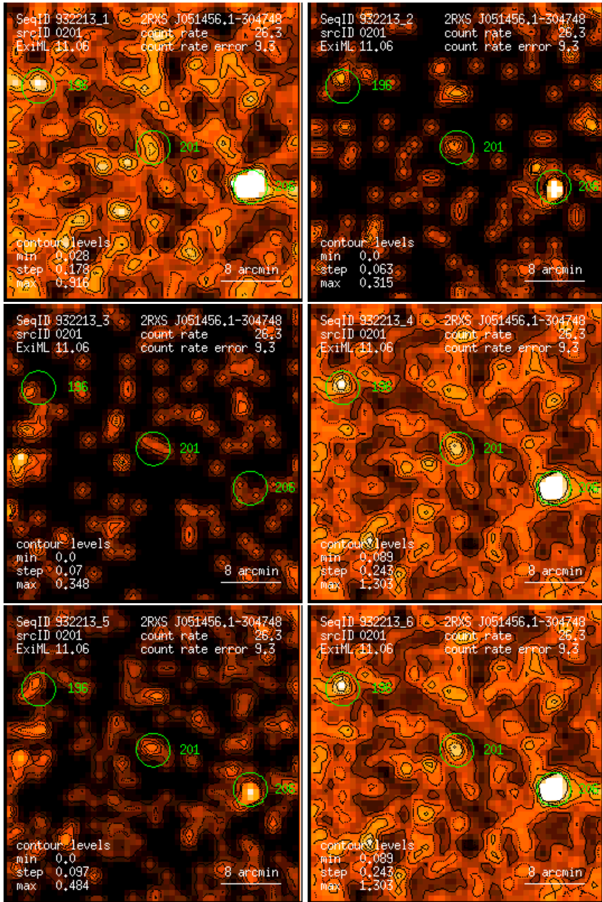
Figure 201: RASS 932213: detection 0201: band rate images, Gaussian filter: (1) PSPC channels 11 – 41, (2) 52 – 90, (3) 91 – 201, (4) 11 – 235, (5) 52 – 201, (6) 11 – 201. Broad band rates in counts/ks. Band rate contour levels in counts/ks/arcmin 2 .
