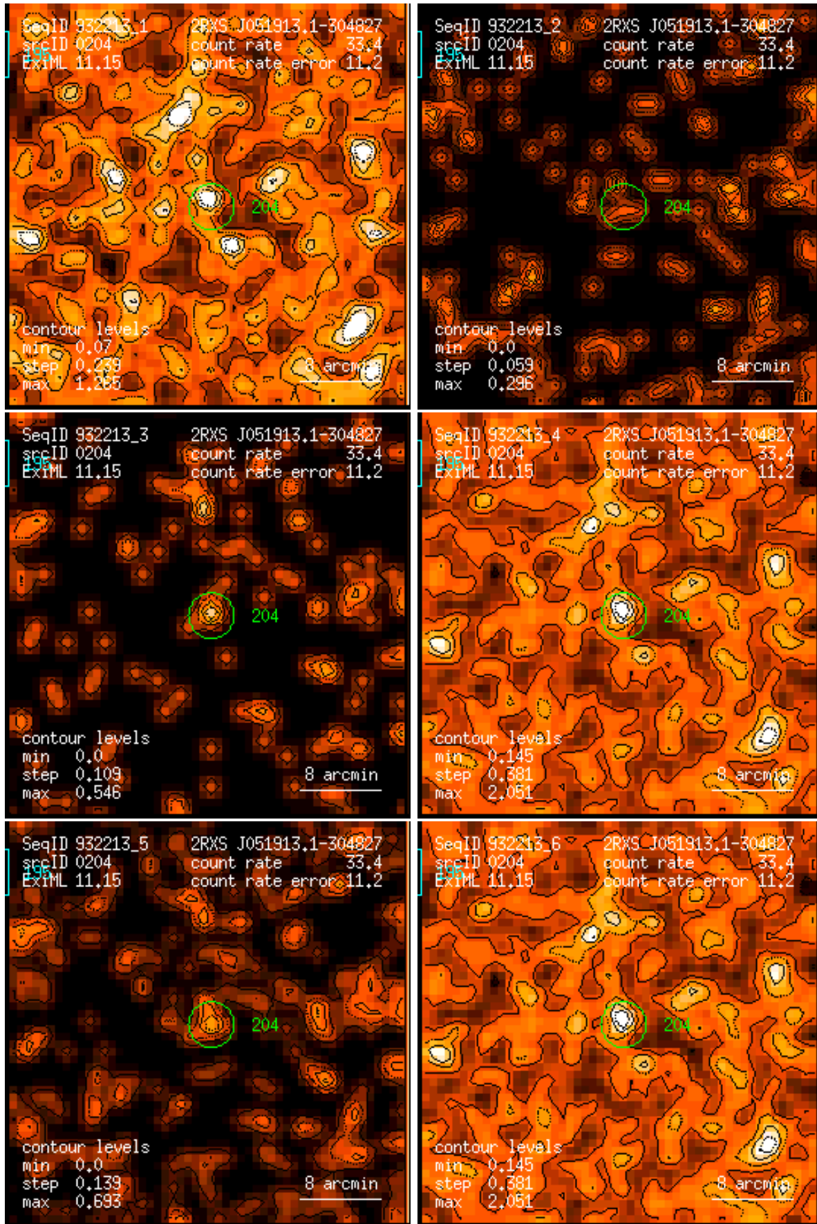
Figure 204: RASS 932213: detection 0204: band rate images, Gaussian filter: (1) PSPC channels 11 – 41, (2) 52 – 90, (3) 91 – 201, (4) 11 – 235, (5) 52 – 201, (6) 11 – 201. Broad band rates in counts/ks. Band rate contour levels in counts/ks/arcmin 2 .
