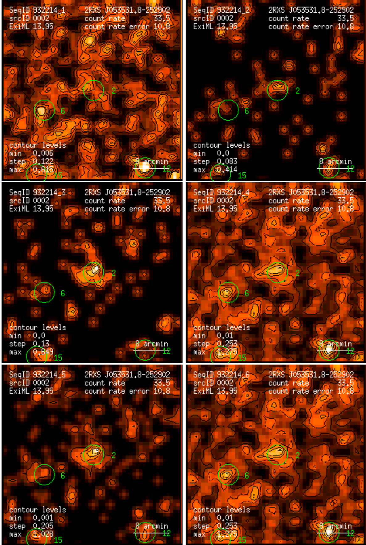
Figure 2: RASS 932214: detection 0002: band rate images, Gaussian filter: (1) PSPC channels 11 – 41, (2) 52 – 90, (3) 91 – 201, (4) 11 – 235, (5) 52 – 201, (6) 11 – 201. Broad band rates in counts/ks. Band rate contour levels in counts/ks/arcmin 2 .
