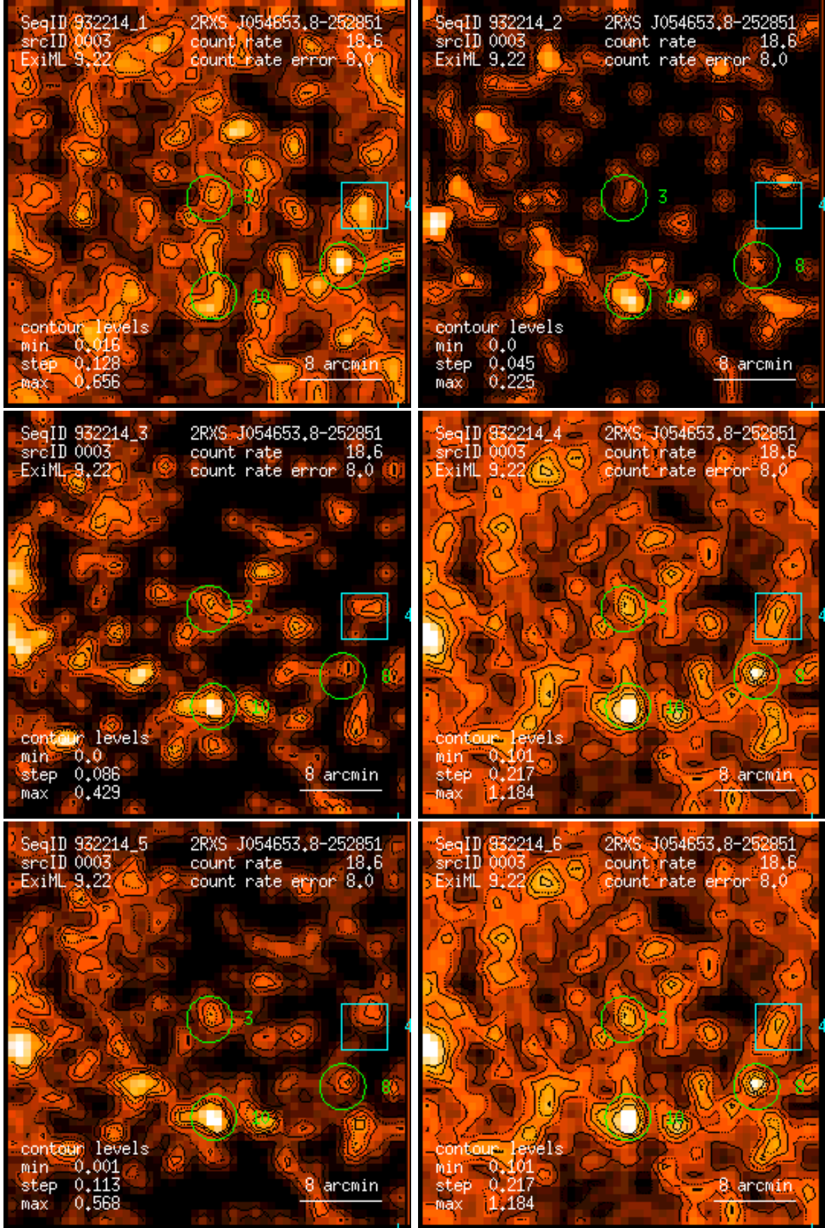
Figure 3: RASS 932214: detection 0003: band rate images, Gaussian filter: (1) PSPC channels 11 – 41, (2) 52 – 90, (3) 91 – 201, (4) 11 – 235, (5) 52 – 201, (6) 11 – 201. Broad band rates in counts/ks. Band rate contour levels in counts/ks/arcmin 2 .
