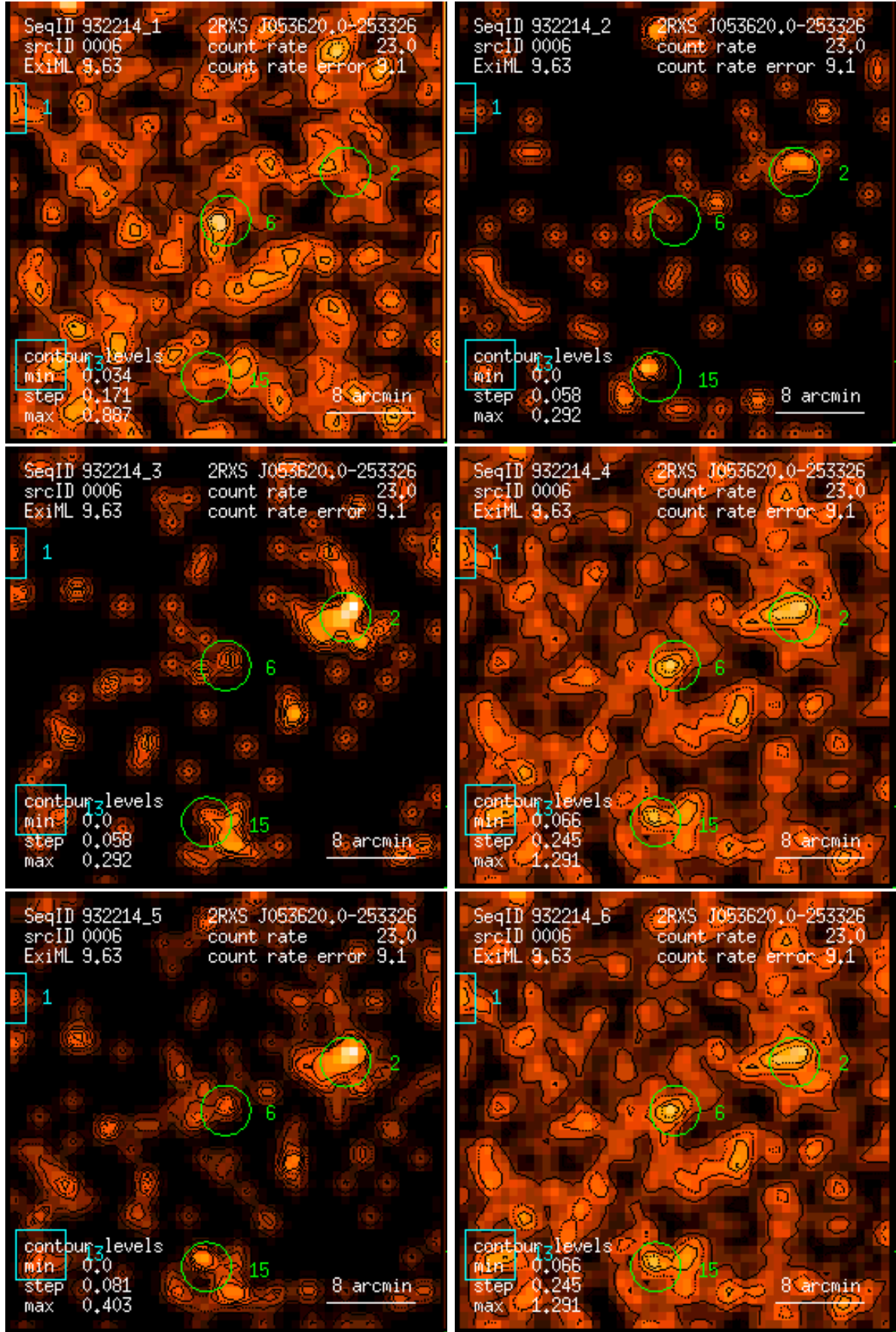
Figure 6: RASS 932214: detection 0006: band rate images, Gaussian filter: (1) PSPC channels 11 – 41, (2) 52 – 90, (3) 91 – 201, (4) 11 – 235, (5) 52 – 201, (6) 11 – 201. Broad band rates in counts/ks. Band rate contour levels in counts/ks/arcmin 2 .
