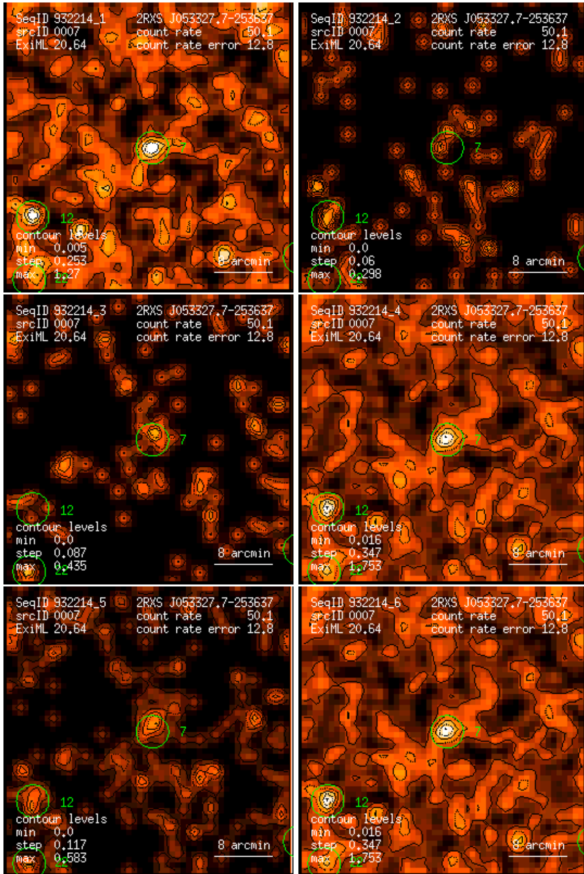
Figure 7: RASS 932214: detection 0007: band rate images, Gaussian filter: (1) PSPC channels 11 – 41, (2) 52 – 90, (3) 91 – 201, (4) 11 – 235, (5) 52 – 201, (6) 11 – 201. Broad band rates in counts/ks. Band rate contour levels in counts/ks/arcmin 2 .
