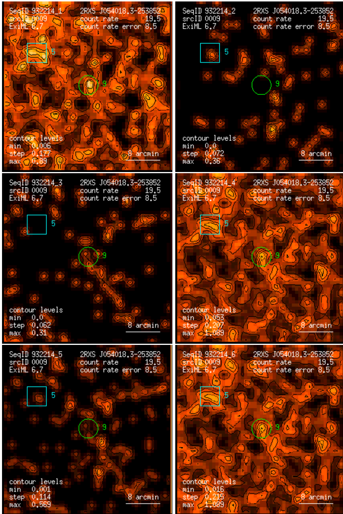
Figure 9: RASS 932214: detection 0009: band rate images, Gaussian filter: (1) PSPC channels 11 – 41, (2) 52 – 90, (3) 91 – 201, (4) 11 – 235, (5) 52 – 201, (6) 11 – 201. Broad band rates in counts/ks. Band rate contour levels in counts/ks/arcmin 2 .
