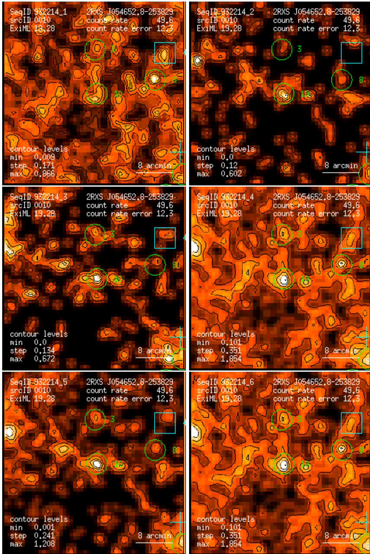
Figure 10: RASS 932214: detection 0010: band rate images, Gaussian filter: (1) PSPC channels 11 – 41, (2) 52 – 90, (3) 91 – 201, (4) 11 – 235, (5) 52 – 201, (6) 11 – 201. Broad band rates in counts/ks. Band rate contour levels in counts/ks/arcmin 2 .
