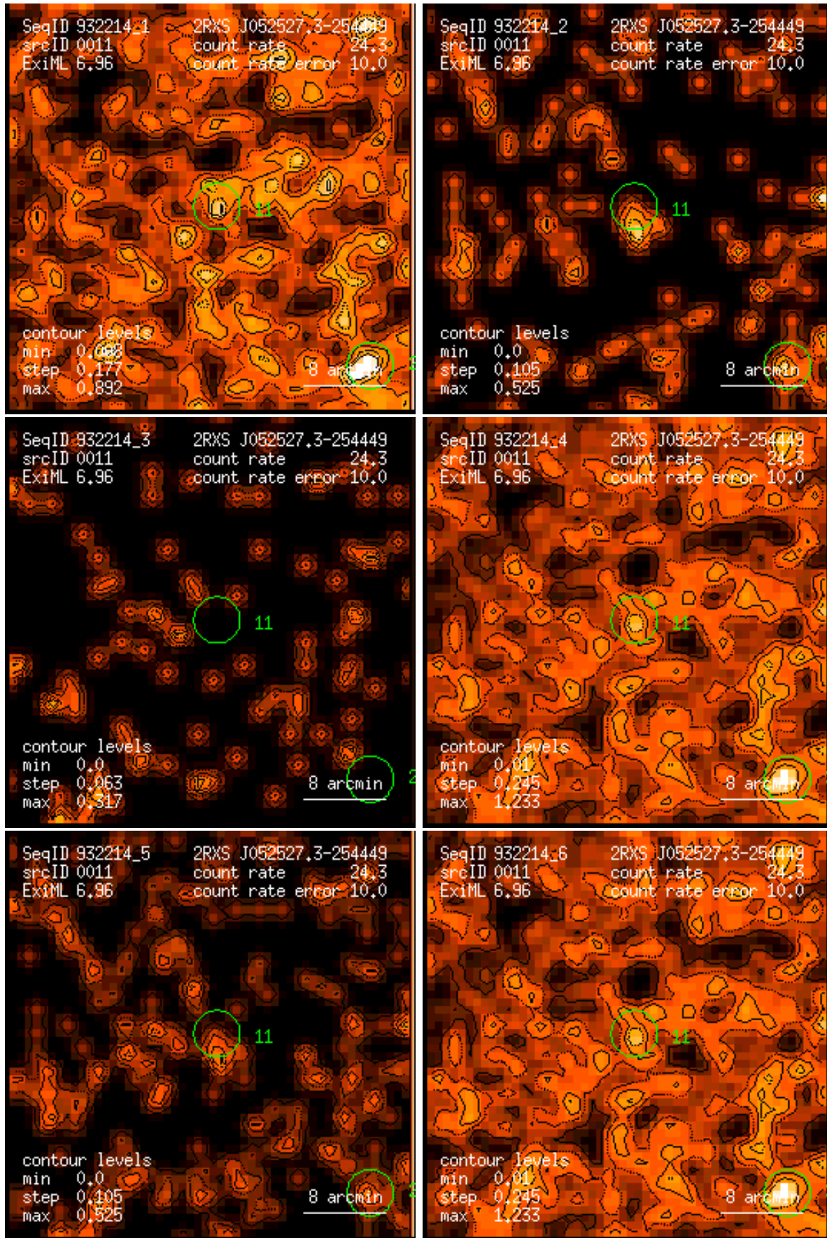
Figure 11: RASS 932214: detection 0011: band rate images, Gaussian filter: (1) PSPC channels 11 – 41, (2) 52 – 90, (3) 91 – 201, (4) 11 – 235, (5) 52 – 201, (6) 11 – 201. Broad band rates in counts/ks. Band rate contour levels in counts/ks/arcmin 2 .
