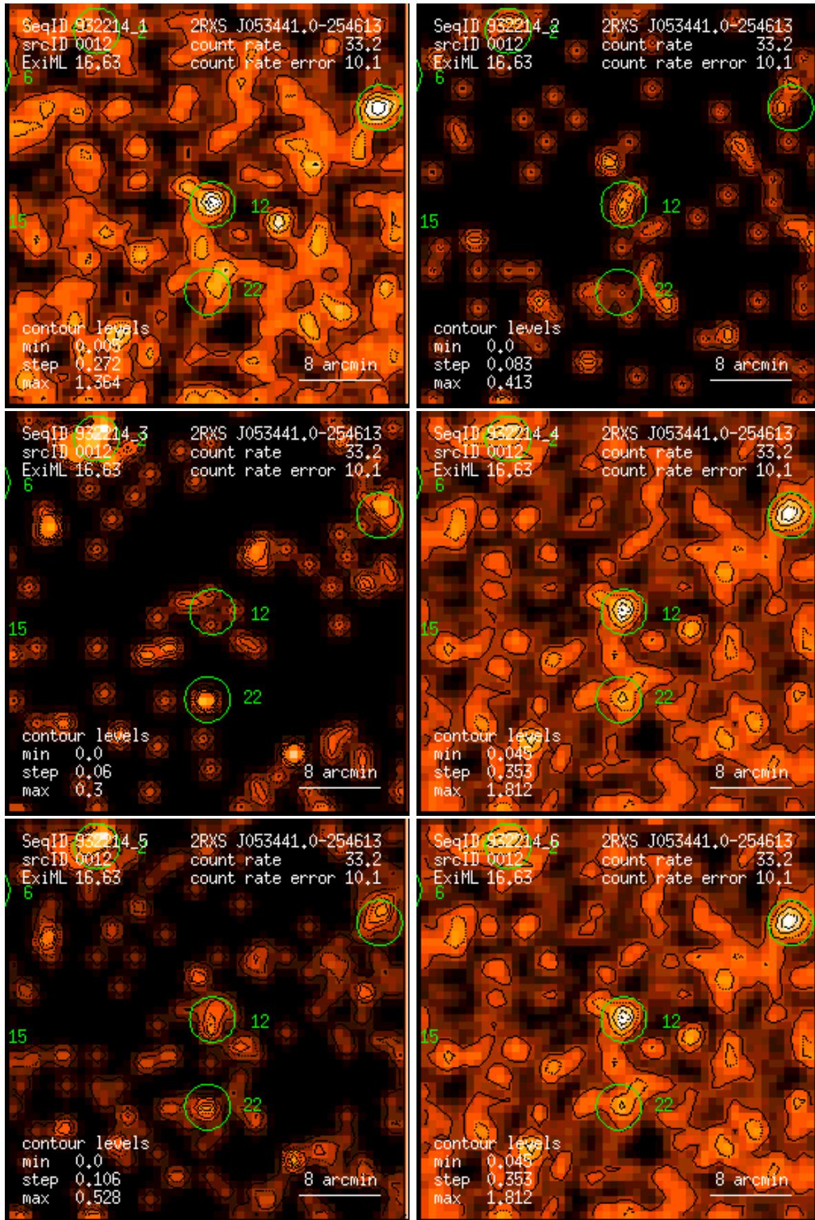
Figure 12: RASS 932214: detection 0012: band rate images, Gaussian filter: (1) PSPC channels 11 – 41, (2) 52 – 90, (3) 91 – 201, (4) 11 – 235, (5) 52 – 201, (6) 11 – 201. Broad band rates in counts/ks. Band rate contour levels in counts/ks/arcmin 2 .
