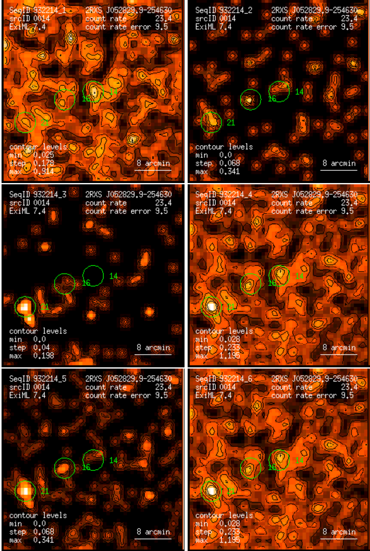
Figure 14: RASS 932214: detection 0014: band rate images, Gaussian filter: (1) PSPC channels 11 – 41, (2) 52 – 90, (3) 91 – 201, (4) 11 – 235, (5) 52 – 201, (6) 11 – 201. Broad band rates in counts/ks. Band rate contour levels in counts/ks/arcmin 2 .
