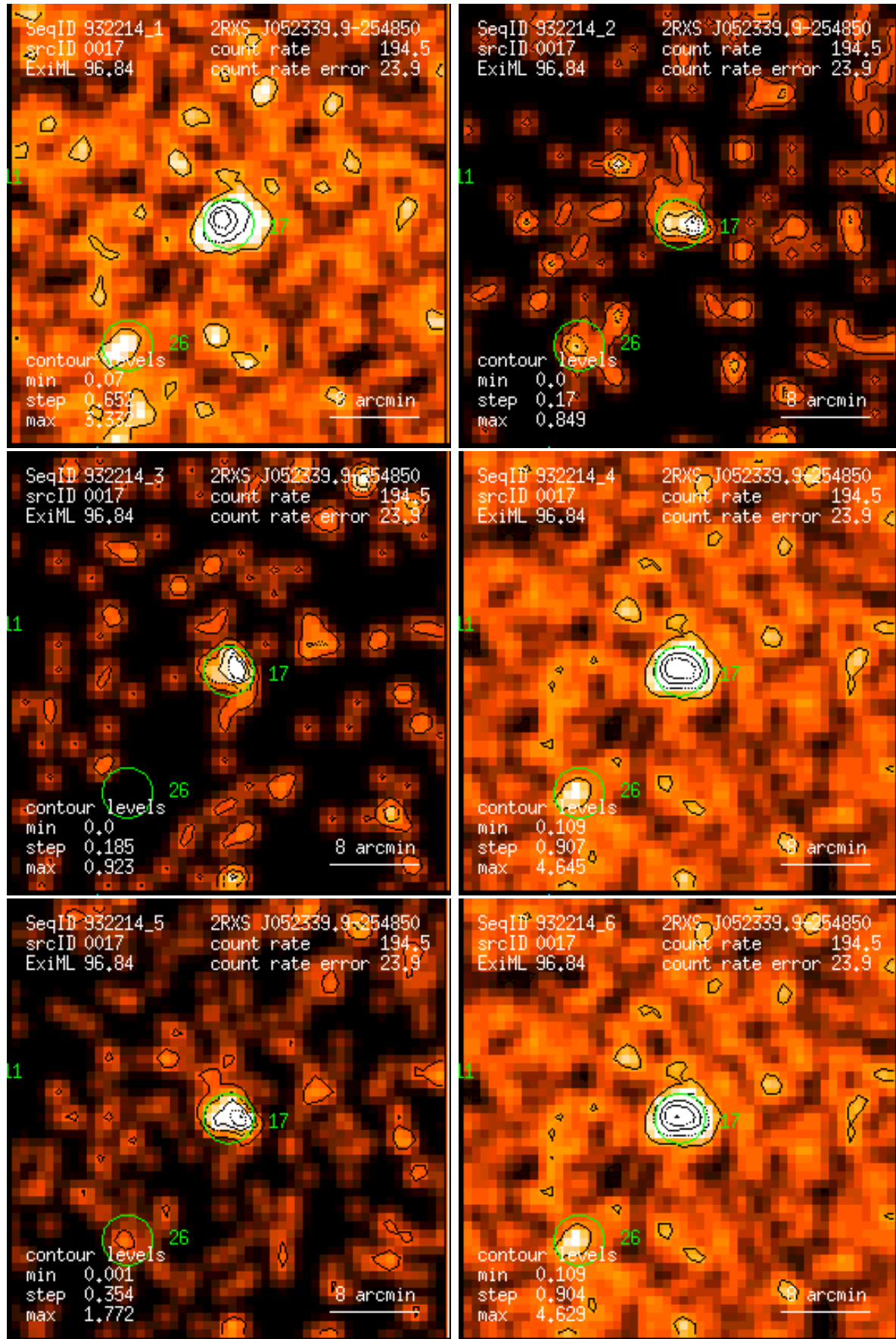
Figure 17: RASS 932214: detection 0017: band rate images, Gaussian filter: (1) PSPC channels 11 – 41, (2) 52 – 90, (3) 91 – 201, (4) 11 – 235, (5) 52 – 201, (6) 11 – 201. Broad band rates in counts/ks. Band rate contour levels in counts/ks/arcmin 2 .
