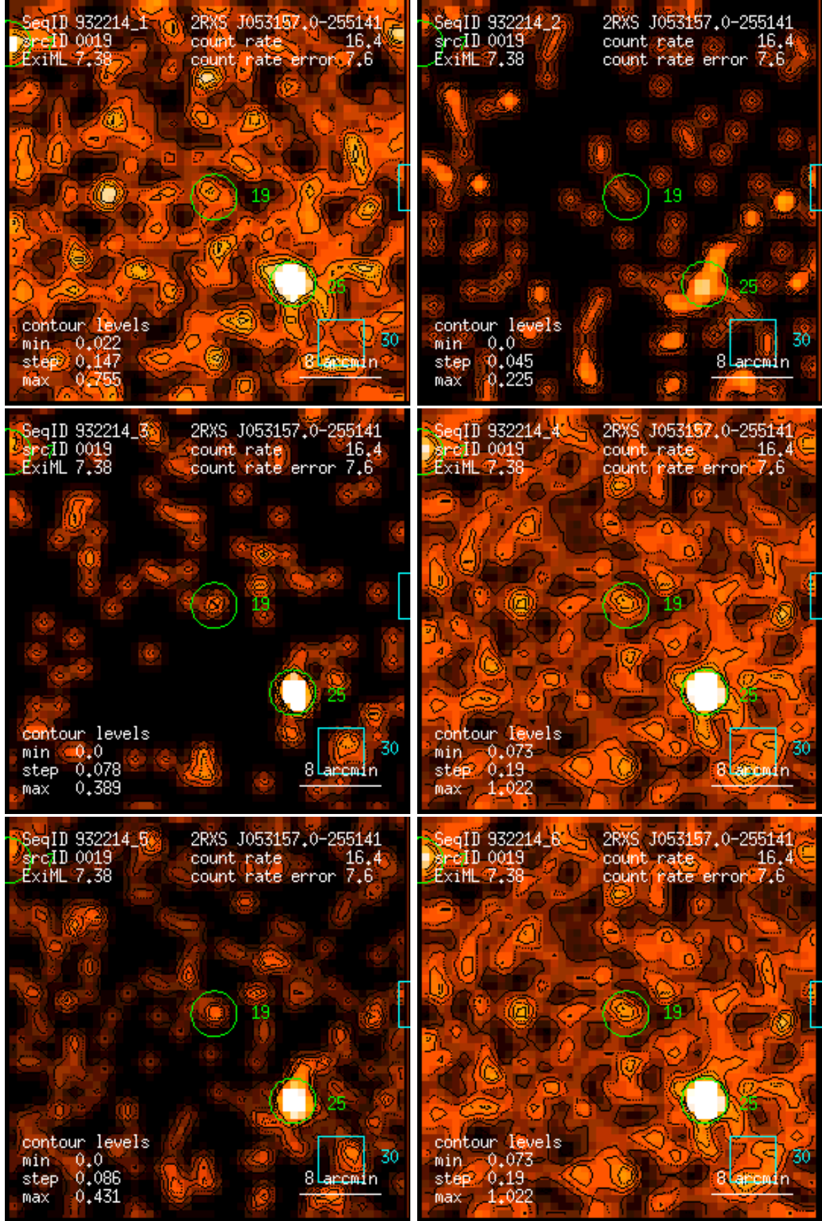
Figure 19: RASS 932214: detection 0019: band rate images, Gaussian filter: (1) PSPC channels 11 – 41, (2) 52 – 90, (3) 91 – 201, (4) 11 – 235, (5) 52 – 201, (6) 11 – 201. Broad band rates in counts/ks. Band rate contour levels in counts/ks/arcmin 2 .
