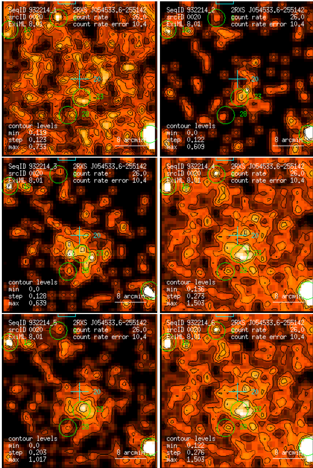
Figure 20: RASS 932214: detection 0020: band rate images, Gaussian filter: (1) PSPC channels 11 – 41, (2) 52 – 90, (3) 91 – 201, (4) 11 – 235, (5) 52 – 201, (6) 11 – 201. Broad band rates in counts/ks. Band rate contour levels in counts/ks/arcmin 2 .
