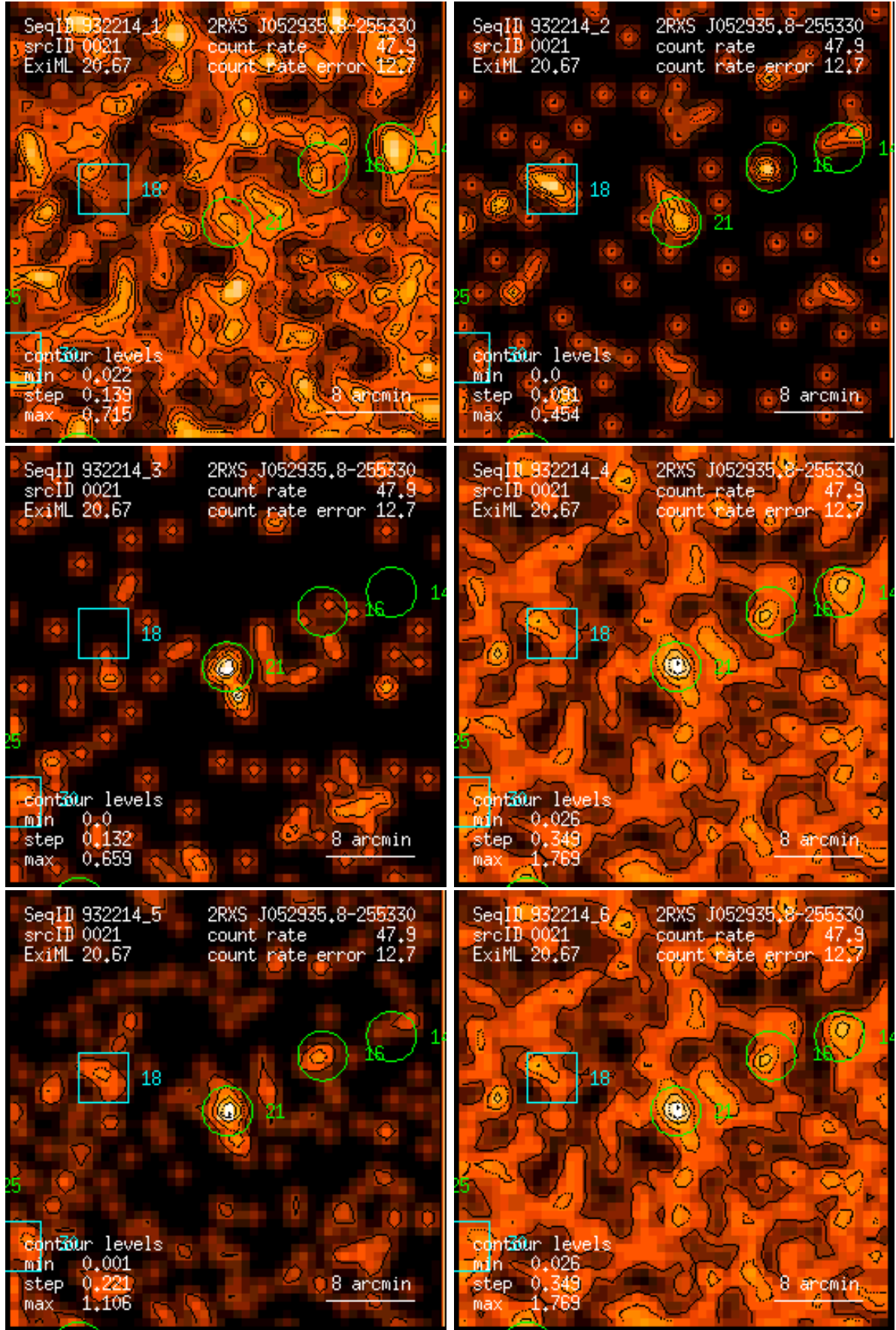
Figure 21: RASS 932214: detection 0021: band rate images, Gaussian filter: (1) PSPC channels 11 – 41, (2) 52 – 90, (3) 91 – 201, (4) 11 – 235, (5) 52 – 201, (6) 11 – 201. Broad band rates in counts/ks. Band rate contour levels in counts/ks/arcmin 2 .
