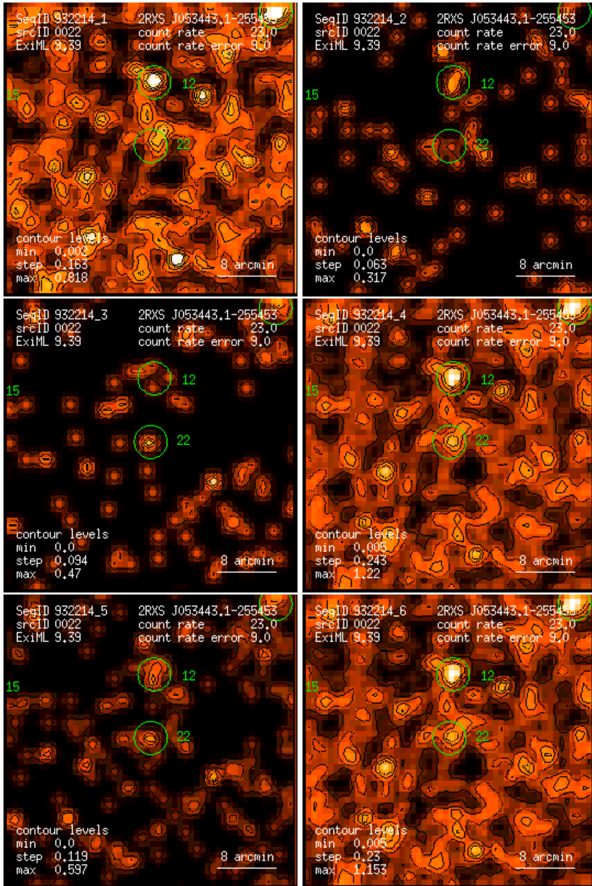
Figure 22: RASS 932214: detection 0022: band rate images, Gaussian filter: (1) PSPC channels 11 – 41, (2) 52 – 90, (3) 91 – 201, (4) 11 – 235, (5) 52 – 201, (6) 11 – 201. Broad band rates in counts/ks. Band rate contour levels in counts/ks/arcmin 2 .
