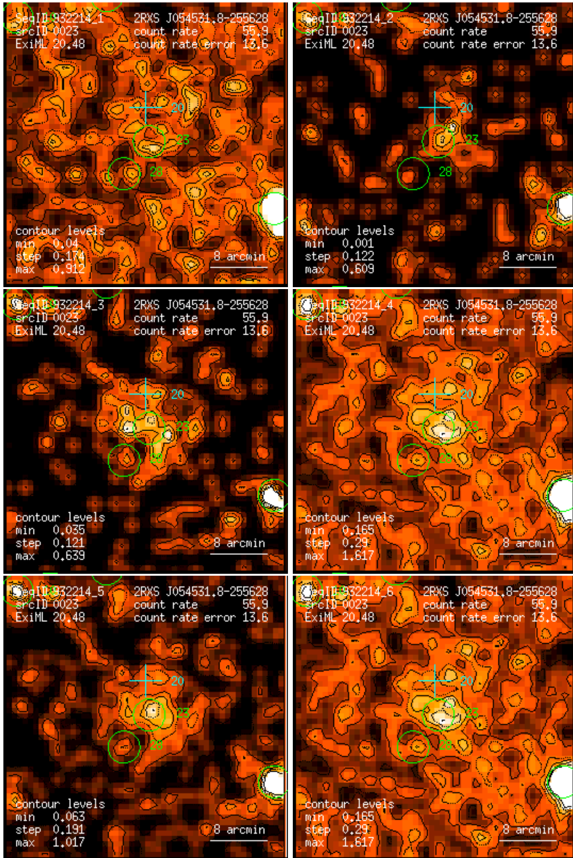
Figure 23: RASS 932214: detection 0023: band rate images, Gaussian filter: (1) PSPC channels 11 – 41, (2) 52 – 90, (3) 91 – 201, (4) 11 – 235, (5) 52 – 201, (6) 11 – 201. Broad band rates in counts/ks. Band rate contour levels in counts/ks/arcmin 2 .
