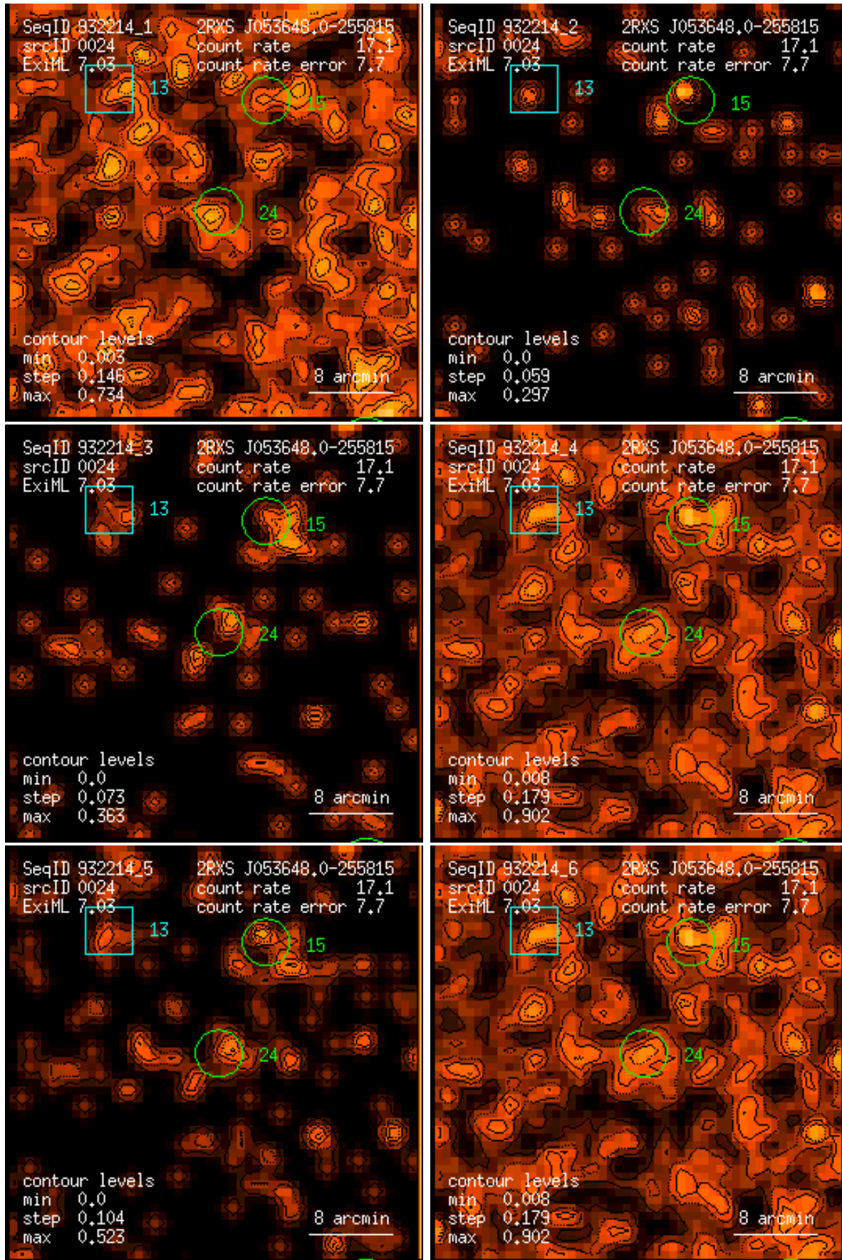
Figure 24: RASS 932214: detection 0024: band rate images, Gaussian filter: (1) PSPC channels 11 – 41, (2) 52 – 90, (3) 91 – 201, (4) 11 – 235, (5) 52 – 201, (6) 11 – 201. Broad band rates in counts/ks. Band rate contour levels in counts/ks/arcmin 2 .
