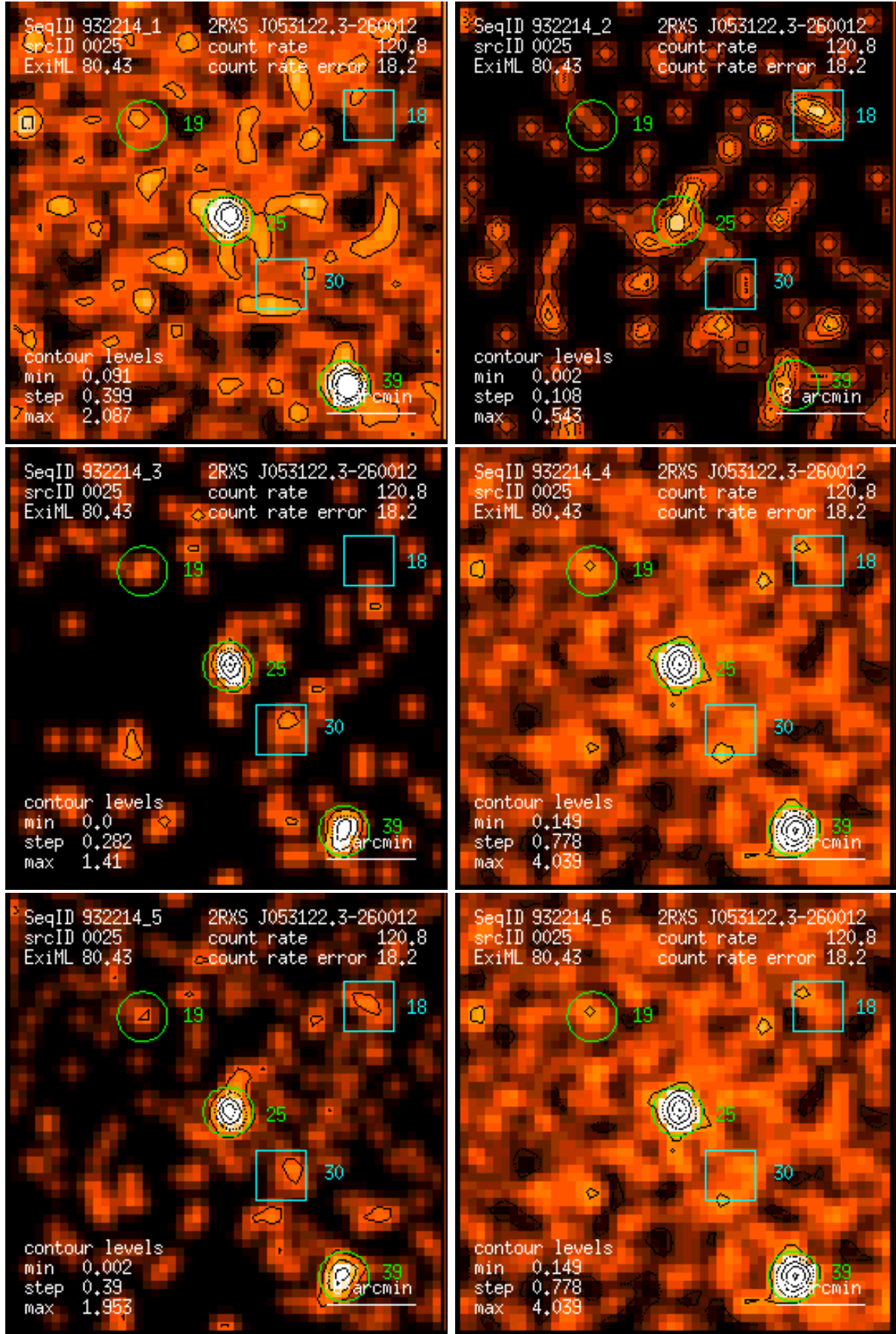
Figure 25: RASS 932214: detection 0025: band rate images, Gaussian filter: (1) PSPC channels 11 – 41, (2) 52 – 90, (3) 91 – 201, (4) 11 – 235, (5) 52 – 201, (6) 11 – 201. Broad band rates in counts/ks. Band rate contour levels in counts/ks/arcmin 2 .
