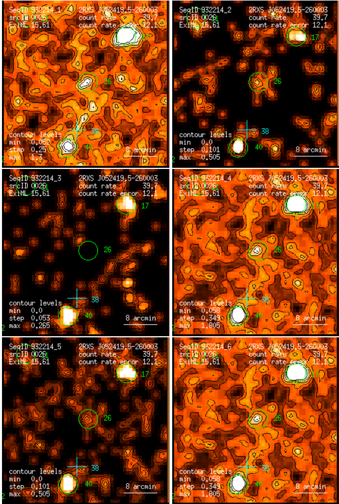
Figure 26: RASS 932214: detection 0026: band rate images, Gaussian filter: (1) PSPC channels 11 – 41, (2) 52 – 90, (3) 91 – 201, (4) 11 – 235, (5) 52 – 201, (6) 11 – 201. Broad band rates in counts/ks. Band rate contour levels in counts/ks/arcmin 2 .
