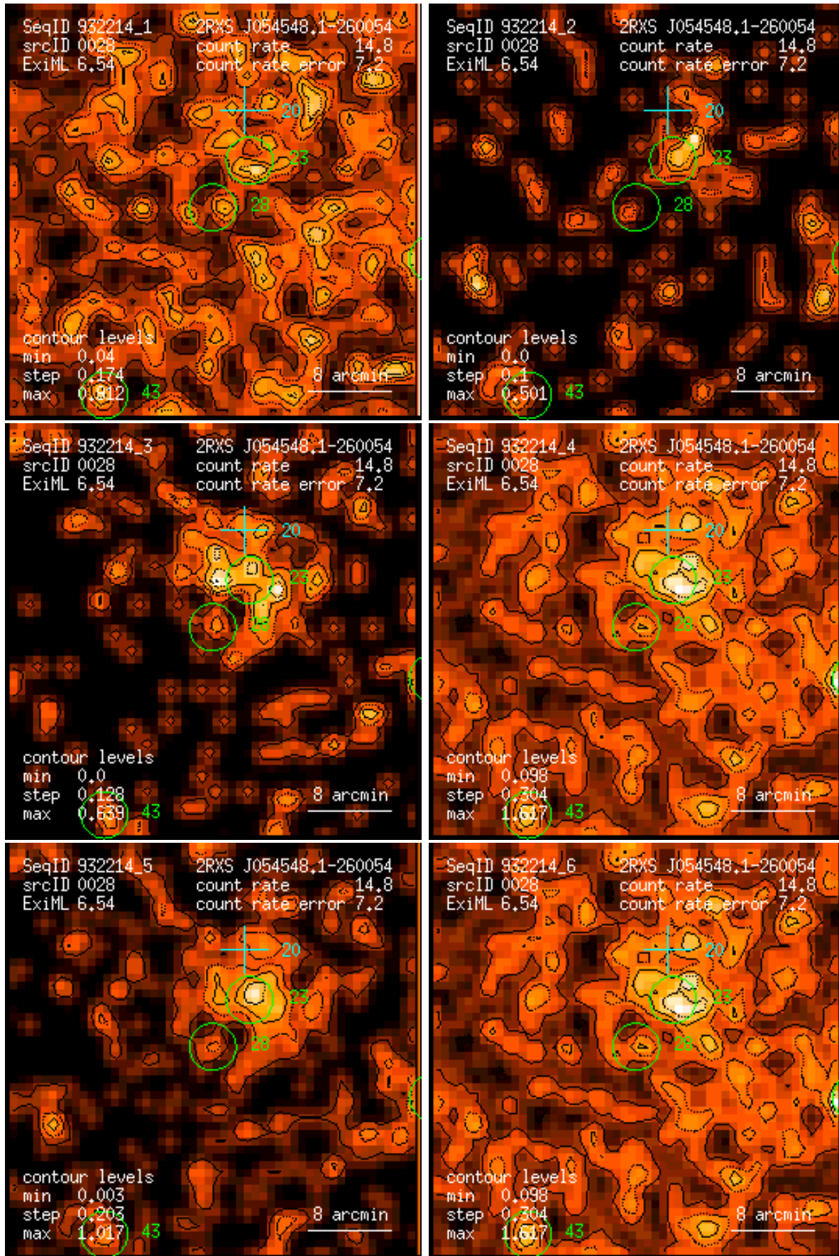
Figure 28: RASS 932214: detection 0028: band rate images, Gaussian filter: (1) PSPC channels 11 – 41, (2) 52 – 90, (3) 91 – 201, (4) 11 – 235, (5) 52 – 201, (6) 11 – 201. Broad band rates in counts/ks. Band rate contour levels in counts/ks/arcmin 2 .
