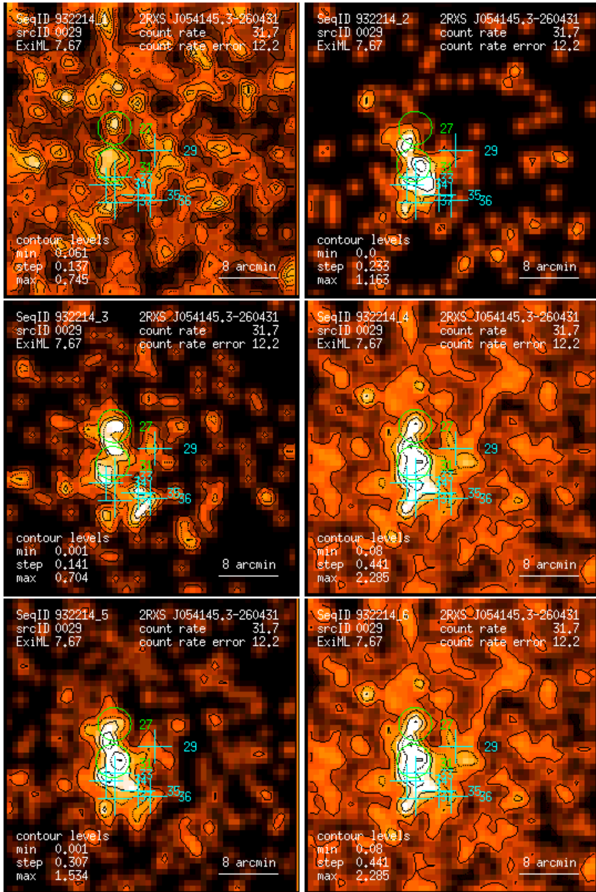
Figure 29: RASS 932214: detection 0029: band rate images, Gaussian filter: (1) PSPC channels 11 – 41, (2) 52 – 90, (3) 91 – 201, (4) 11 – 235, (5) 52 – 201, (6) 11 – 201. Broad band rates in counts/ks. Band rate contour levels in counts/ks/arcmin 2 .
