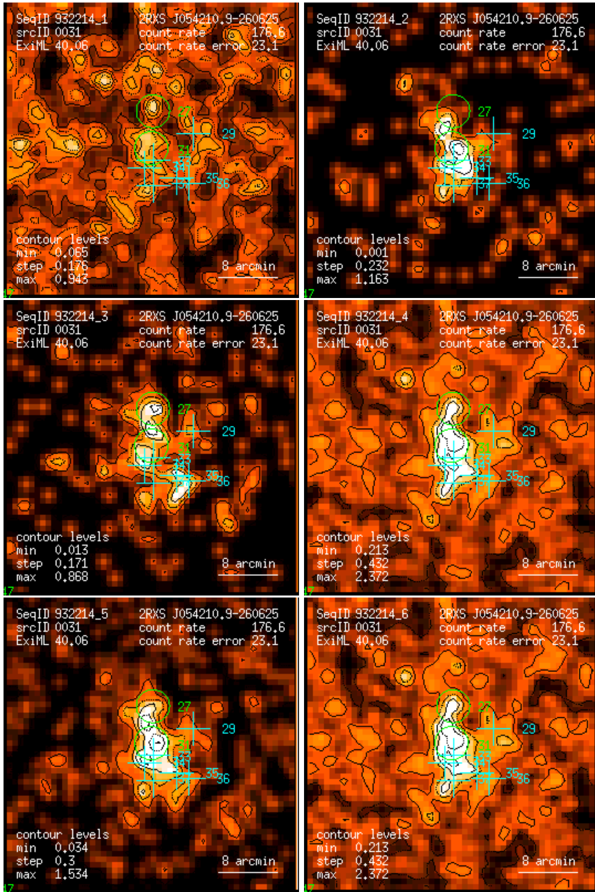
Figure 31: RASS 932214: detection 0031: band rate images, Gaussian filter: (1) PSPC channels 11 – 41, (2) 52 – 90, (3) 91 – 201, (4) 11 – 235, (5) 52 – 201, (6) 11 – 201. Broad band rates in counts/ks. Band rate contour levels in counts/ks/arcmin 2 .
