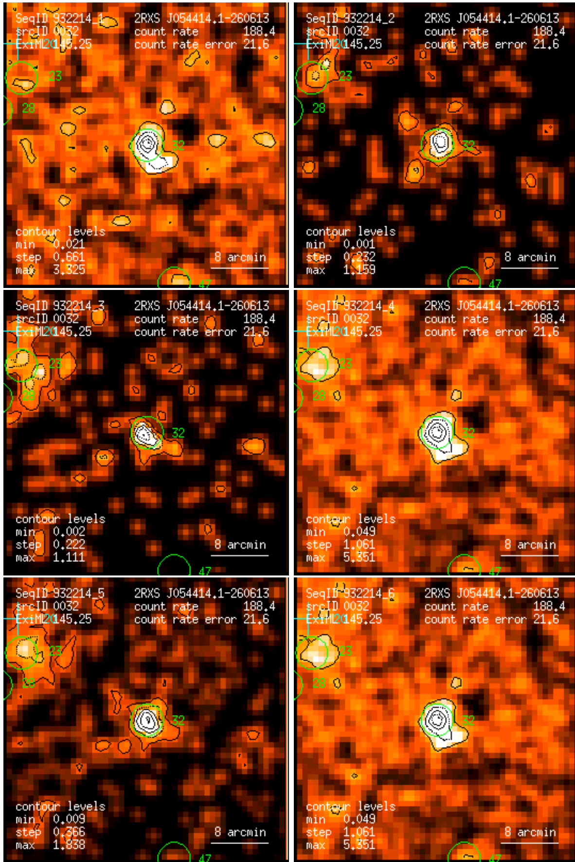
Figure 32: RASS 932214: detection 0032: band rate images, Gaussian filter: (1) PSPC channels 11 – 41, (2) 52 – 90, (3) 91 – 201, (4) 11 – 235, (5) 52 – 201, (6) 11 – 201. Broad band rates in counts/ks. Band rate contour levels in counts/ks/arcmin 2 .
